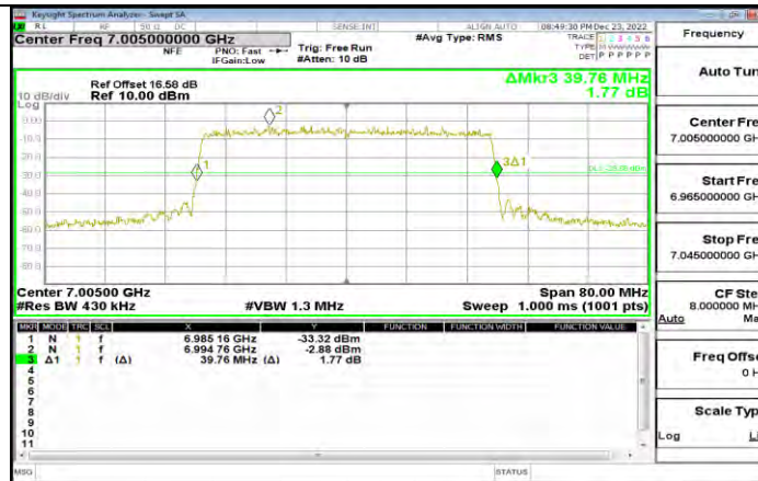
11AX40MIMO Ant1_7005
