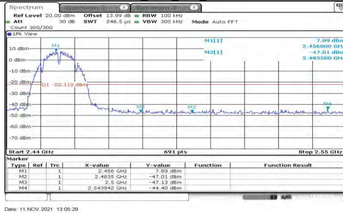
11B_Ant1_High_2457
