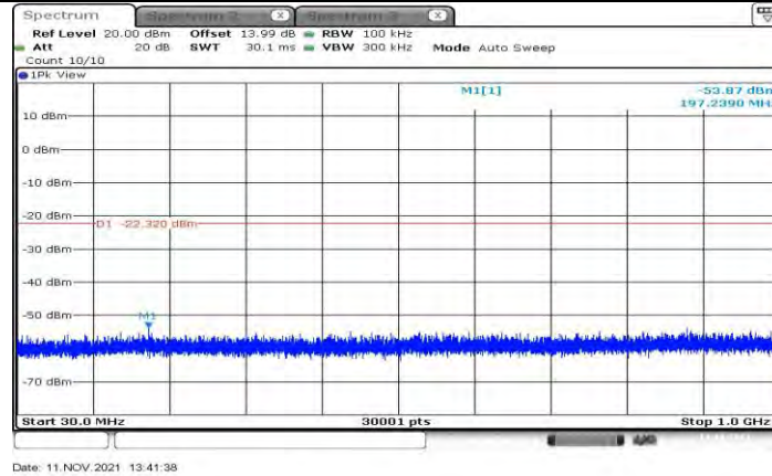
11G_Ant1_2457_30~1000
