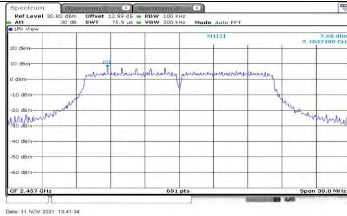
11G_Ant1_2457_0~Reference
