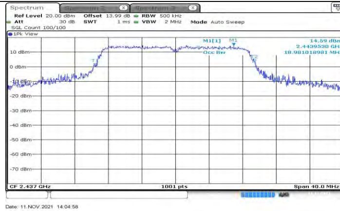
11N20SISO Ant1 2437
