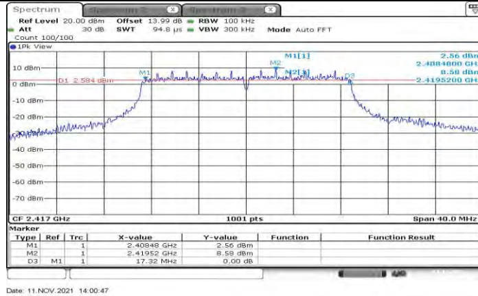
11N20SISO Ant1 2417
