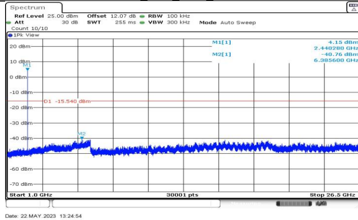
LE 1M_Ant1_2440_1000~26500
