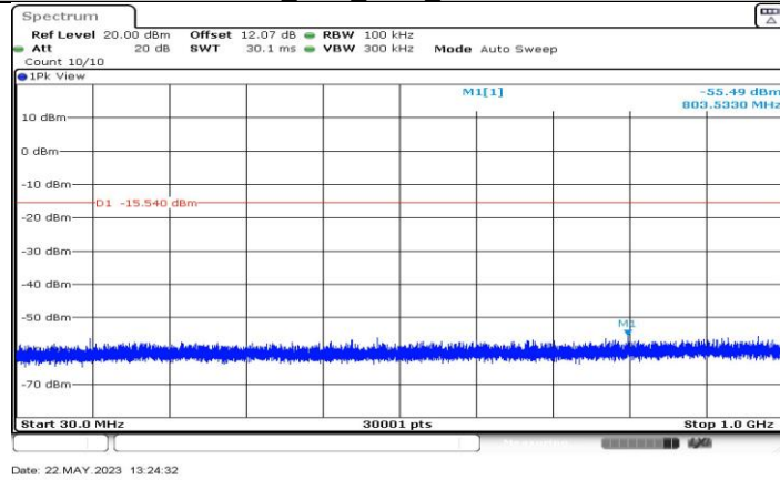
LE 1M_Ant1_2440_30~1000
