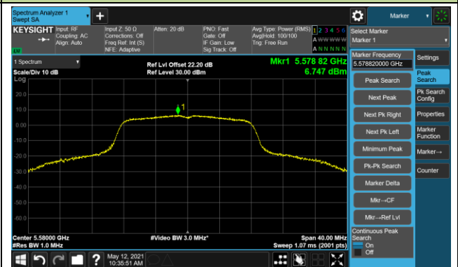
Channel 64 (5580MHz)
