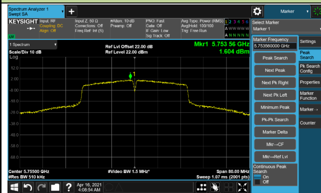
802.11ac-VHT80 Power Spectral Density – Ant 1/Ant 0 + 1
