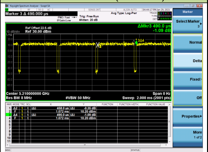
802.11ac-VHT80 (T=458.0us)
