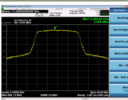
Channel 60 (5300MHz)
