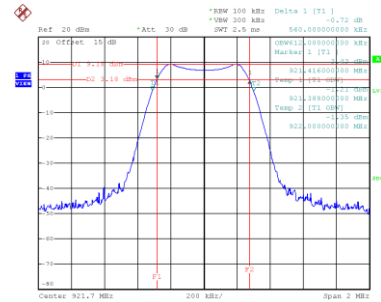
CH01 6 dB Bandwidth
