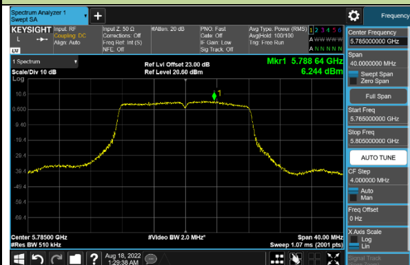
Channel 157 (5785MHz)
