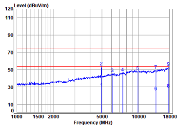
Right BT_DH5_TX_CH_78_Horizontal
