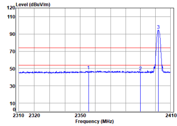
Left BT_DH5_TX_CH_00_Vertical
