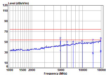
Right BT_DH5_TX_CH_78_Vertical
