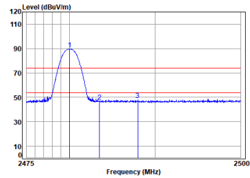
Left BT_DH5_TX_CH_78_Vertical
