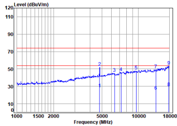
Right BT_DH5_TX_CH_00_Horizontal
