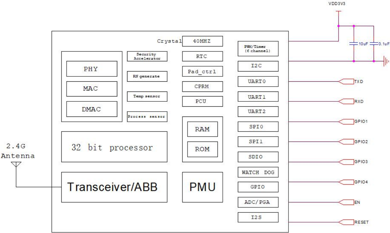
LA-WE3L Wi-Fi Module functional block diagram
