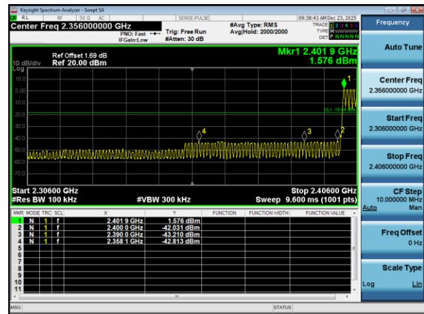
Band-edge Emission
