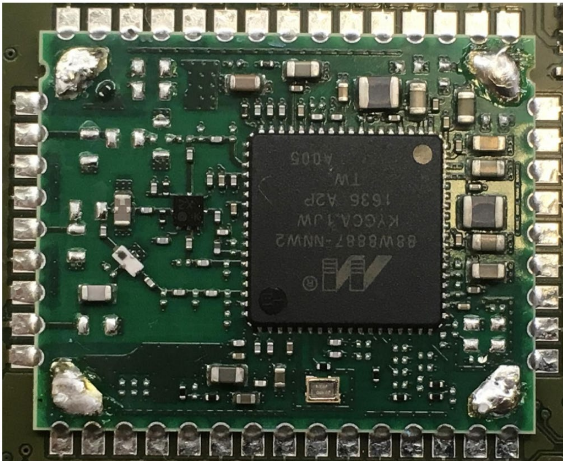
162097_27.jpg: UGKZ7A1001A module without shielding*
