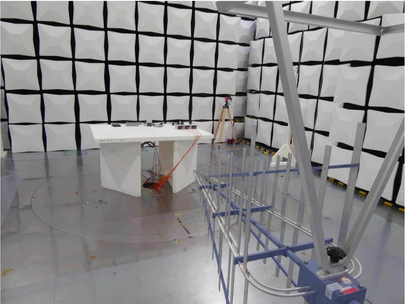
Test setup from 30 MHz to 1 GHz
