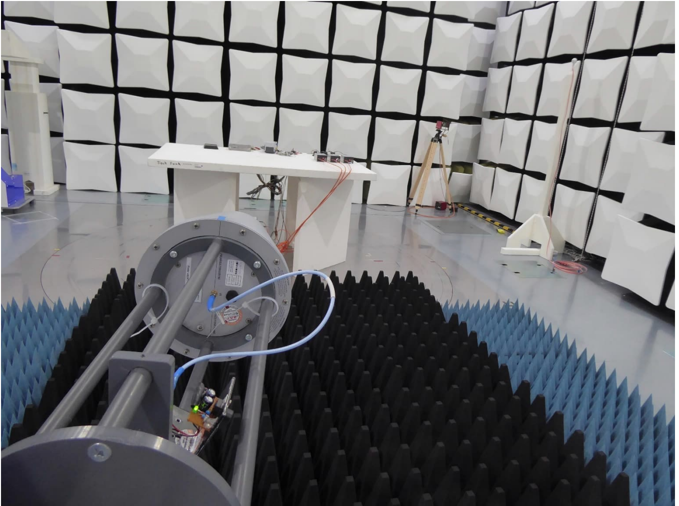
Test setup from 1 GHz to 13 GHz
