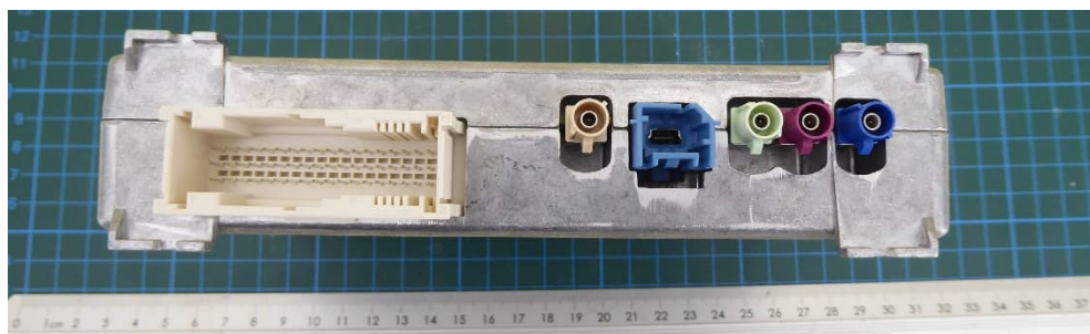
Host Rear view with ports
