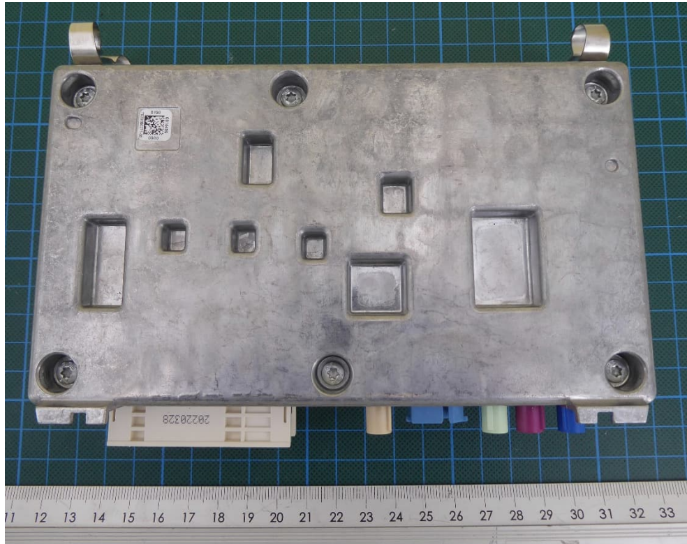
Host Bottom view
