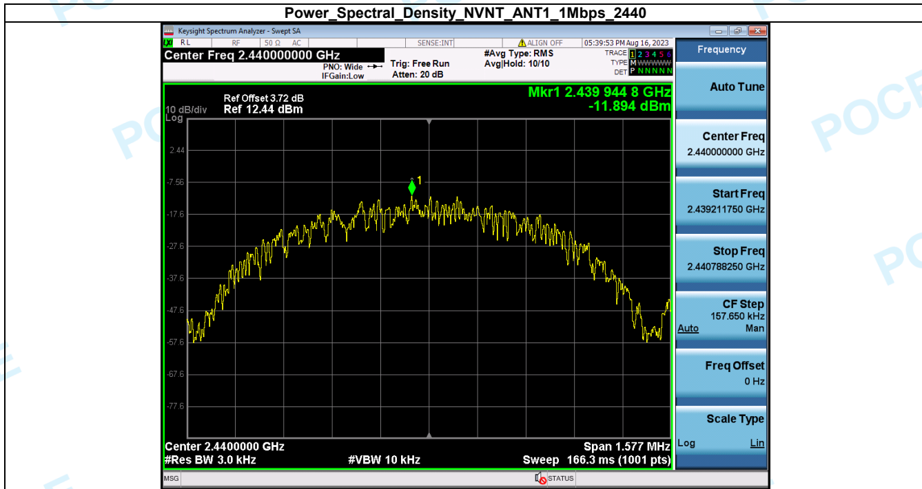
Power_Spectral_Density_NVNT_ANT1_1Mbps_2440
