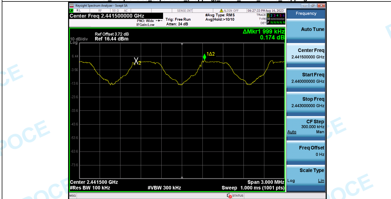
Carrier_Frequencies_Separation_(Hopping)_NVNT_ANT1_1-DH5_Hopping
