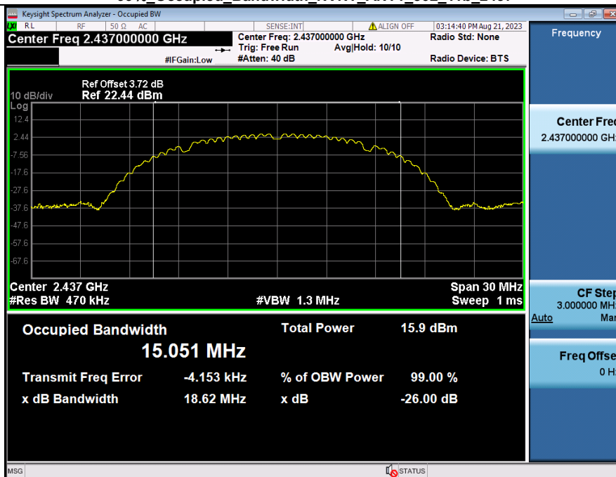
99% Occupied Bandwidth_NVNT_ANT1_802_11b_2437
