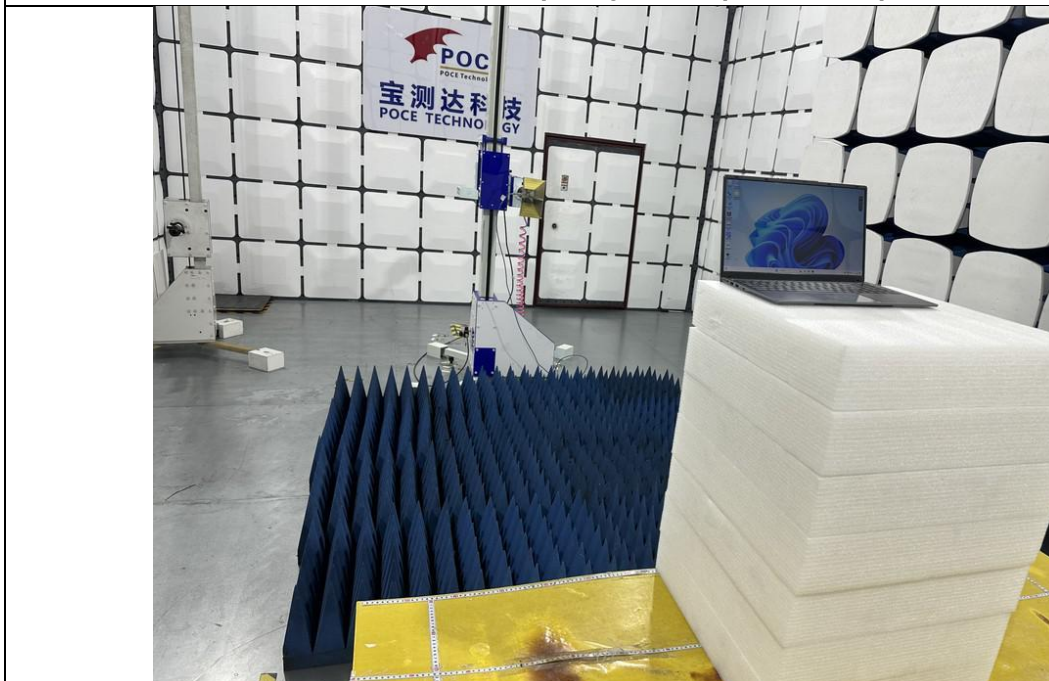
Emissions in frequency bands (above 1GHz)
