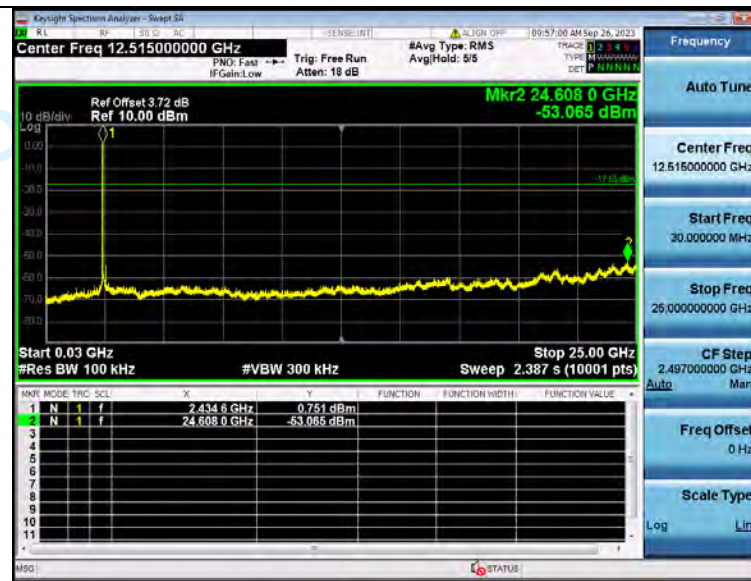
2 Spurious Emission NVNT ANT2 802 11b 2437
