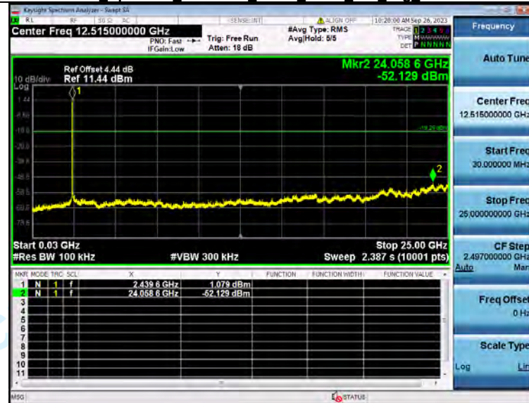
2 Spurious Emission NVNT ANT2 802 11g 2437
