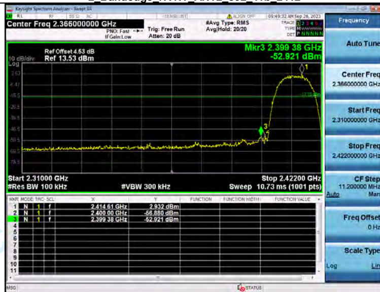
2 Bandedge NVNT ANT2 802 11b 2412
