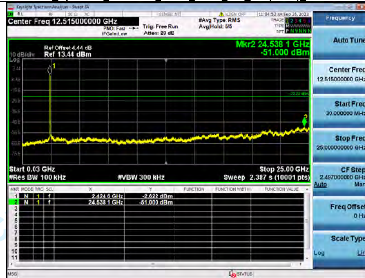
2 Spurious Emission NVNT ANT2 802 11n(HT40) 2437
