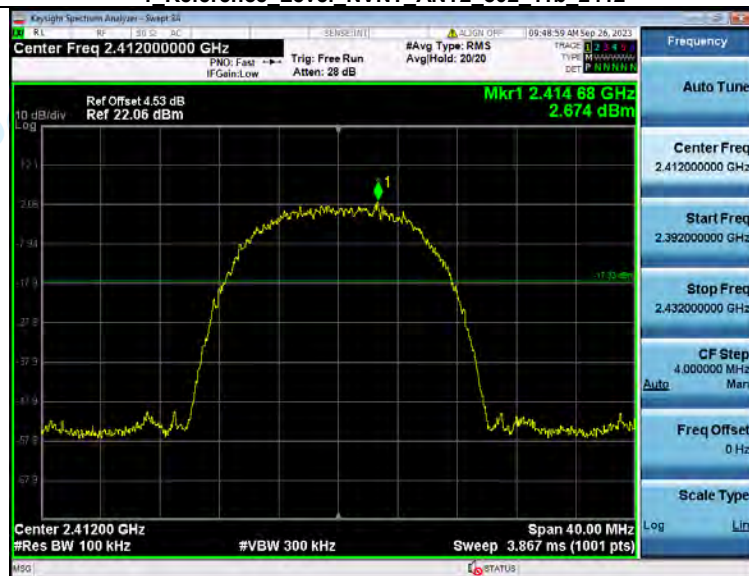
2_Bandedge_NVNT_ANT1_802_11b_2412
