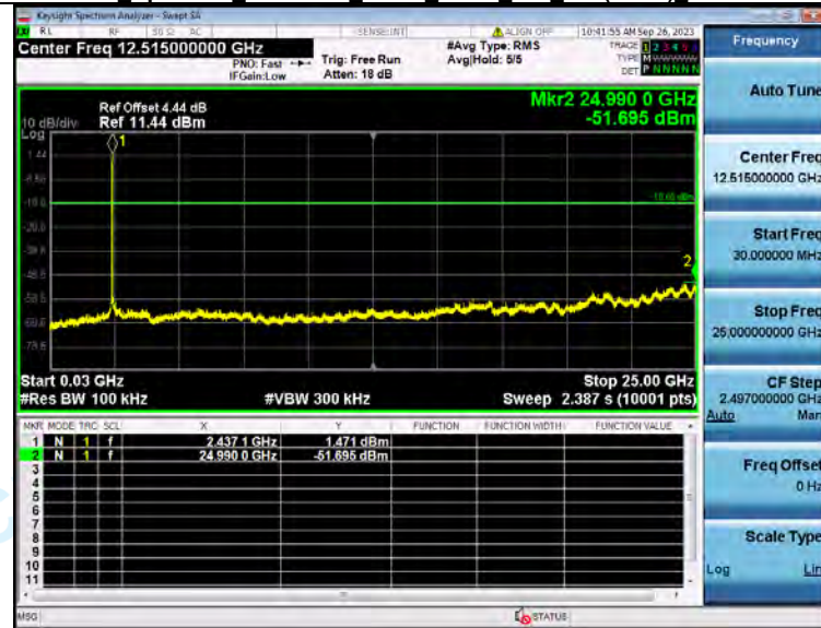
2 Spurious Emission NVNT ANT2 802 11n(HT20) 2437
