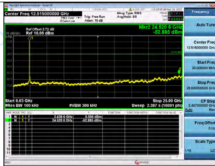
2 Spurious Emission NVNT ANT2 802 11g 2437
