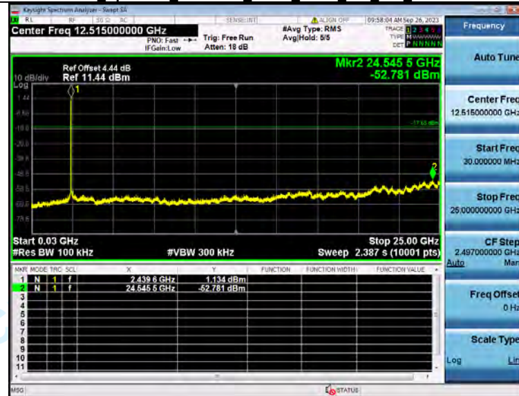
2 Spurious Emission NVNT ANT2 802 11b 2437
