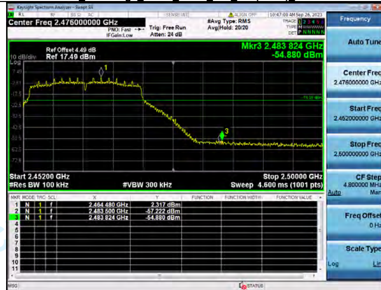
2 Bandedge NVNT ANT2 802 11n(HT20) 2462
