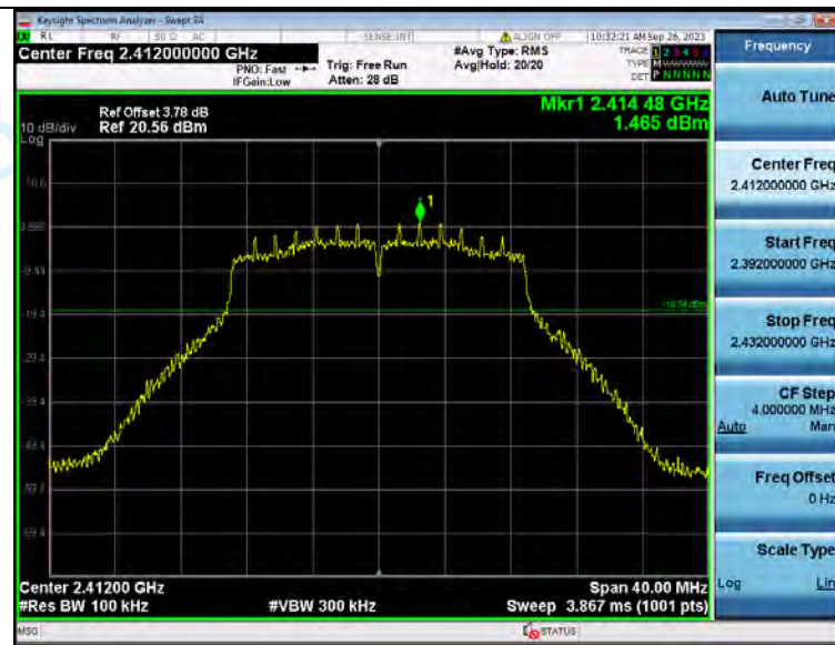
1 Reference Level NVNT ANT2 802 11n(HT20) 2412
