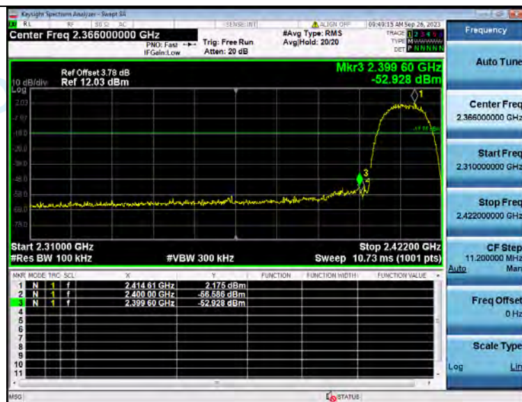
2 Bandedge NVNT ANT2 802 11b 2412
