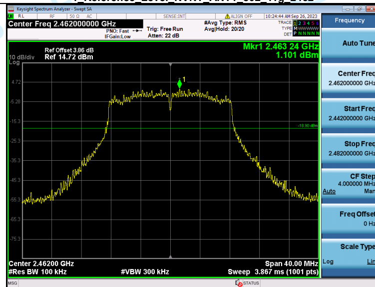
1 Reference Level NVNT ANT2 802 11g 2462
