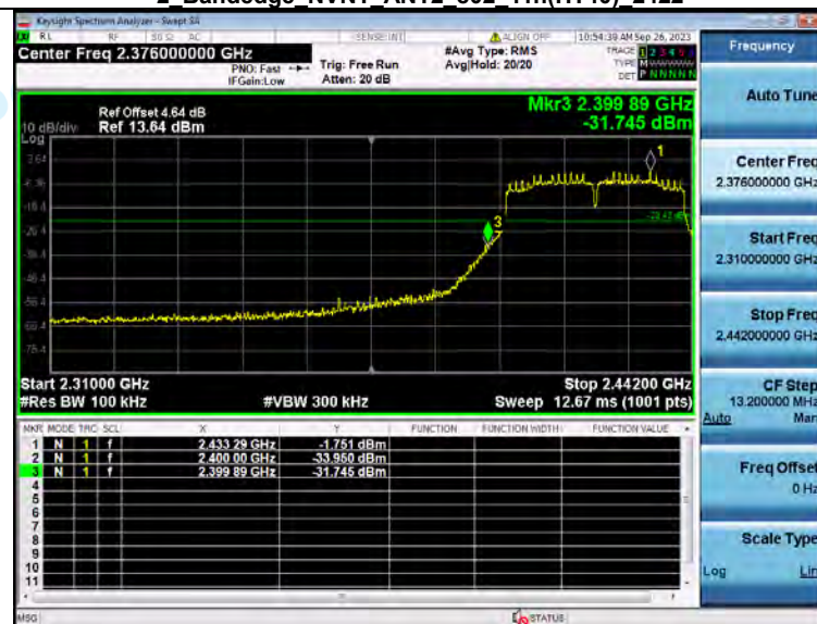
2 Bandedge NVNT ANT2 802 11n(HT40) 2422
