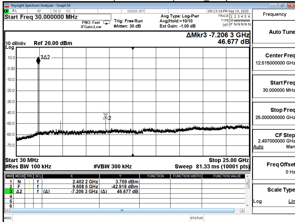
Channel 00 (30MHz-25GHz)- GFSK_1Mbps
