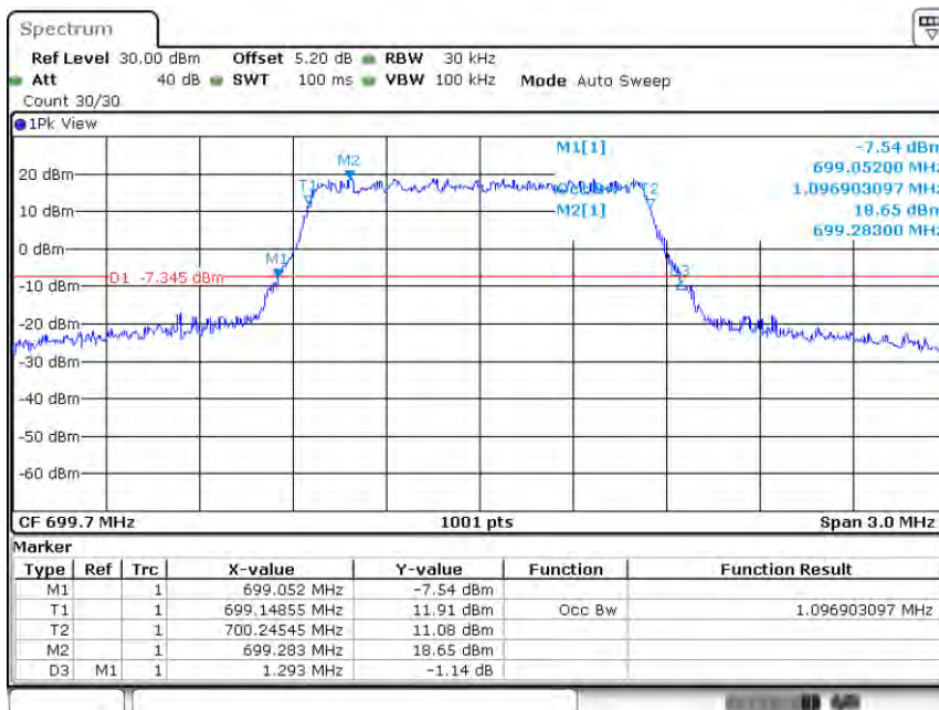
Band12-1.4MHz-QPSK-23017-6RB#0-1.097
