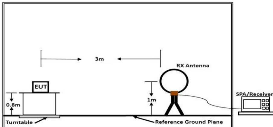
Below 30MHz
