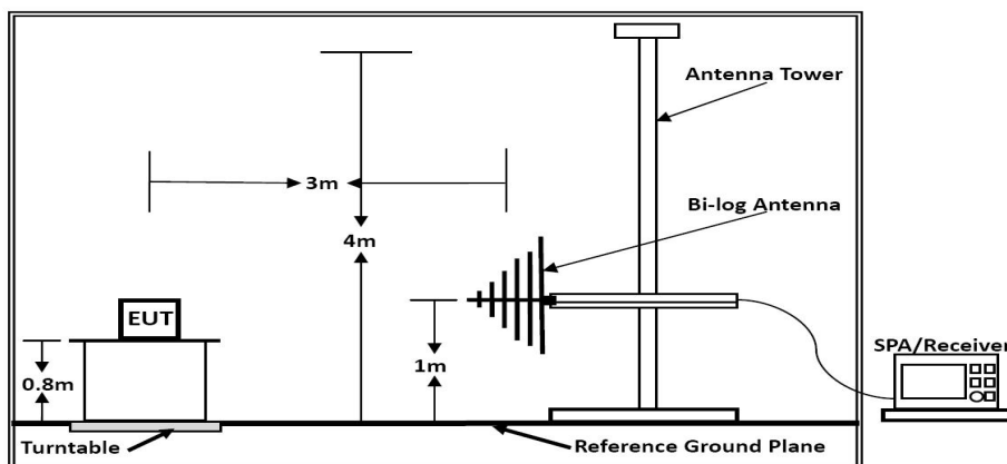
Below 1GHz
