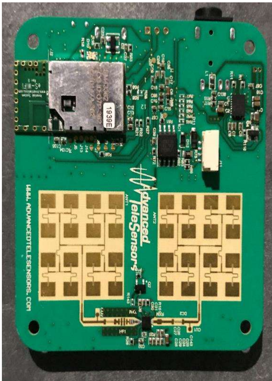
Antenna/Top Side
