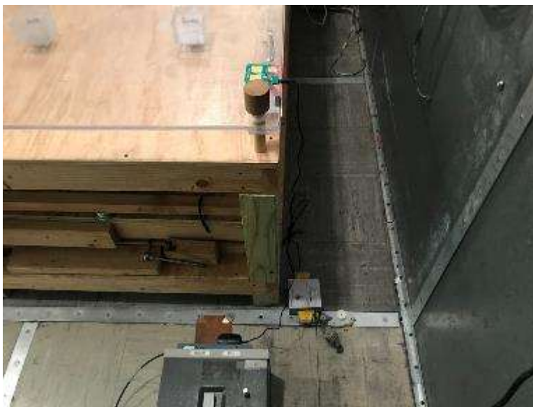
Mains Conducted
