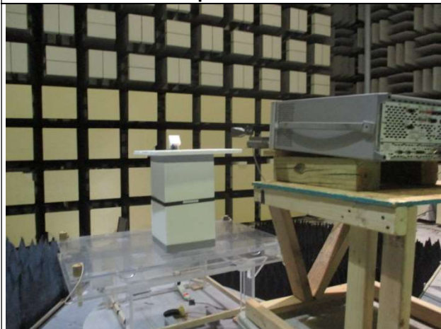
RE Test Setup – 18GHz – 26.5GHz
