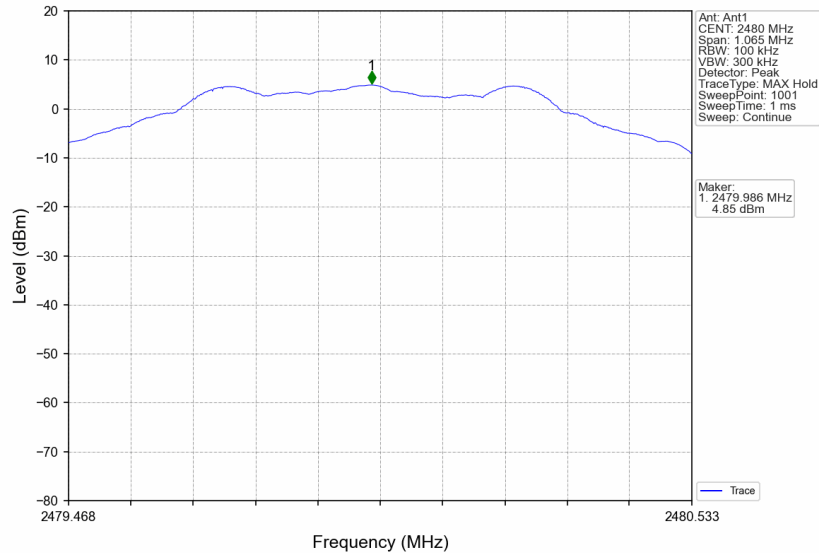
1M_HCH_2480MHz_Ant1_NTNV
