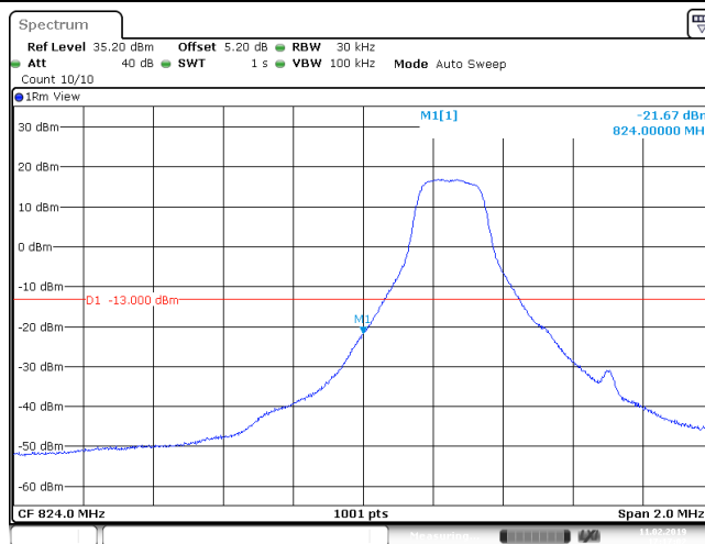
BAND 26_1.4MHz_QPSK_26797_1RB#0
