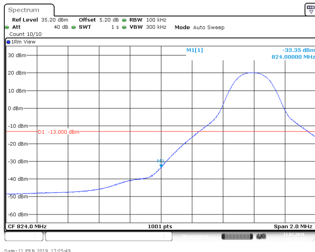
BAND 26 10MHz 16QAM 26840 50RB#0
