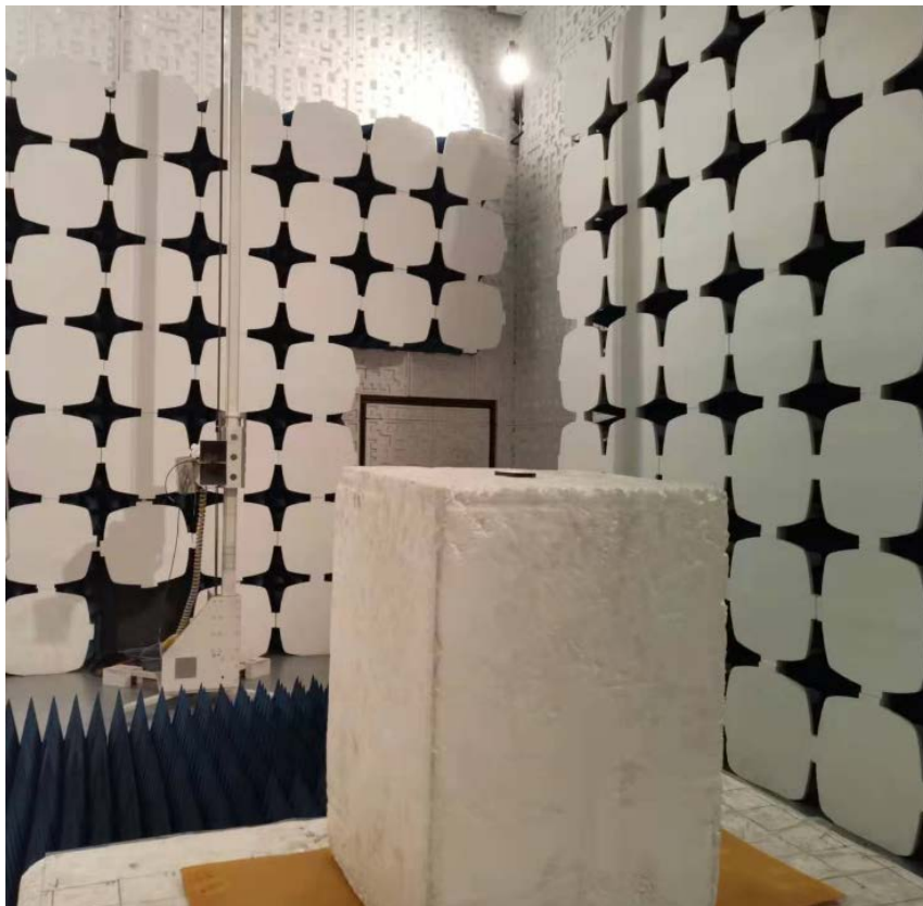
Above 1GHz
