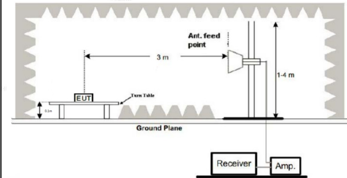
Above 1GHz
