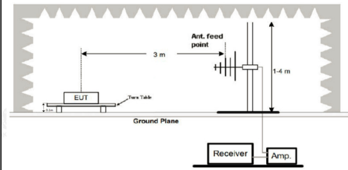
Above 1GHz
