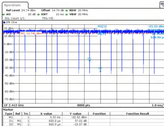
Test Graph_IEEE802.11 ax (HE20) Duty Cycle:
