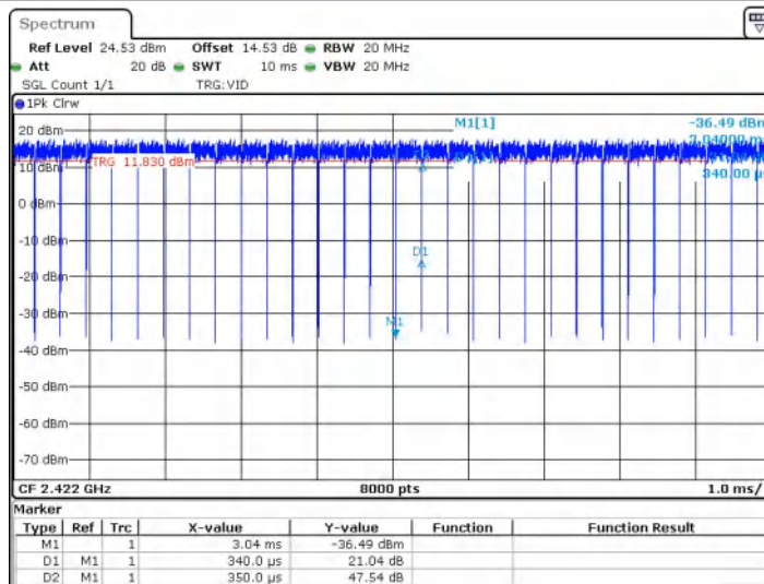
Test Graph_IEEE802.11 ax (HE40) Duty Cycle:
