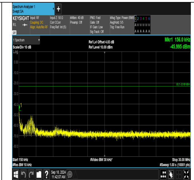
GPRS850-190-5-0.15~30MHz-PASS
