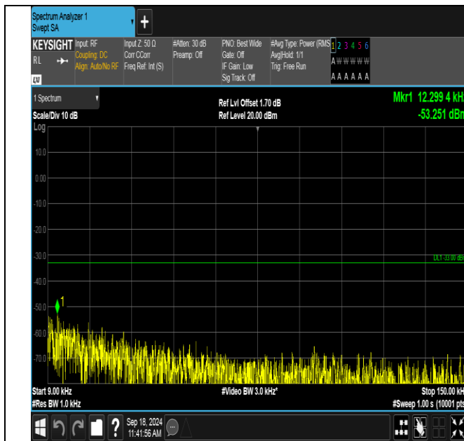
GPRS850-190-5-0.009~0.15MHz-PASS
