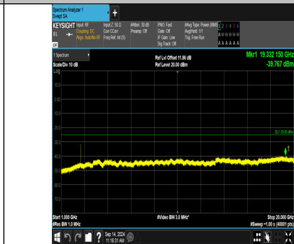
Band41_5MHz_QPSK_40590_25RB#0_1000~20000_1000~20000
