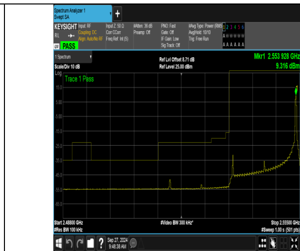
Band41_20MHz_16QAM_40140_1RB#99
