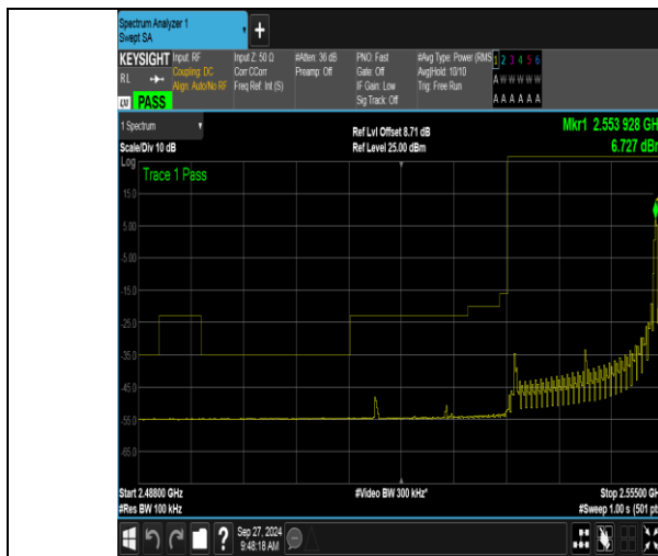
Band41_20MHz_QPSK_40140_1RB#99
