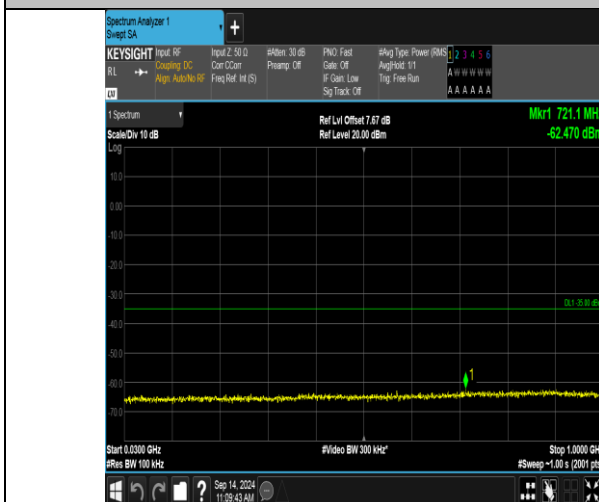
Band41_5MHz_QPSK_40065_1RB#24_30~1000_30~1000
