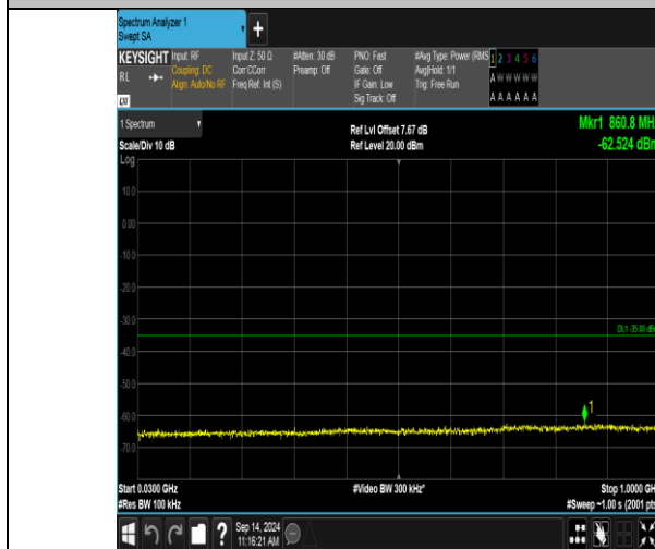
Band41_5MHz_QPSK_40590_25RB#0_30~1000_30~1000
