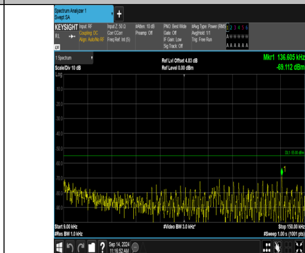
Band41_5MHz_16QAM_40590_25RB#0_0.009~0.15_0.009~0.15
