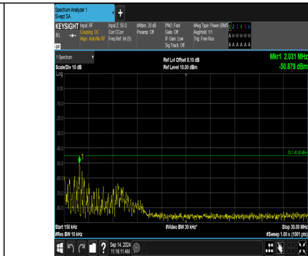
Band41_5MHz_QPSK_40590_25RB#0_0.15~30_0.15~30
