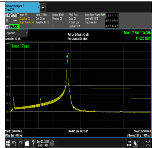
Band41_15MHz_16QAM_41165_1RB#74
