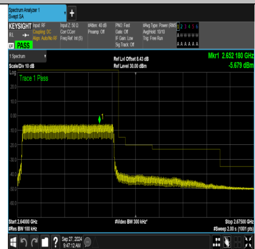
Band41_15MHz_16QAM_41165_75RB#0
