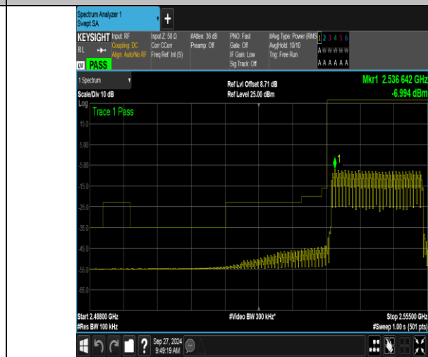
Band41_20MHz_16QAM_40140_100RB#0
