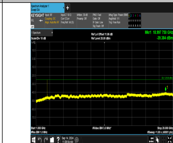
Band41_5MHz_QPSK_40065_1RB#24_1000~20000_1000~20000
