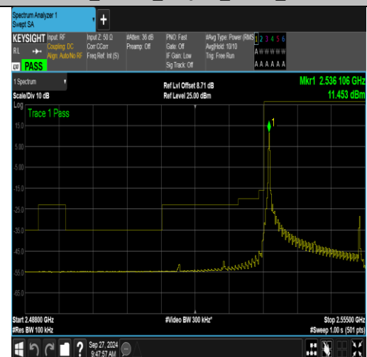
Band41_20MHz_16QAM_40140_1RB#0
