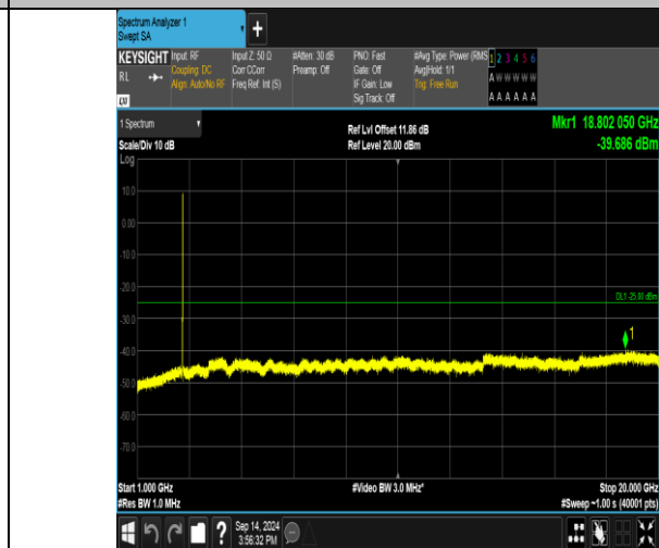
Band41_20MHz_QPSK_41140_100RB#0_1000~20000_1000~20000
