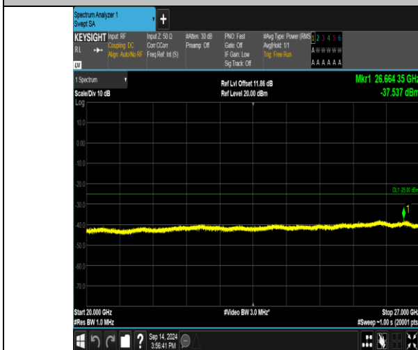
Band41_20MHz_QPSK_41140_100RB#0_20000~27000_20000~27000
