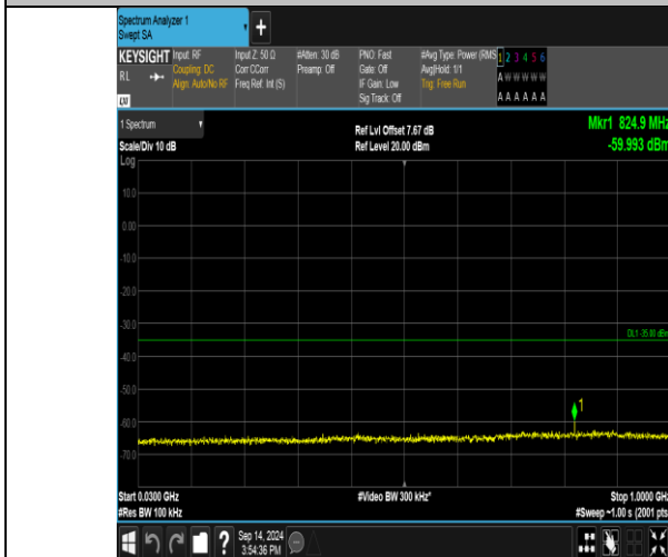
Band41_20MHz_QPSK_41140_1RB#99_30-1000_30-1000
