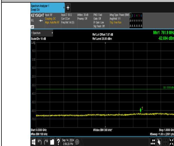
Band41_20MHz_QPSK_41140_100RB#0_30~1000_30~1000
