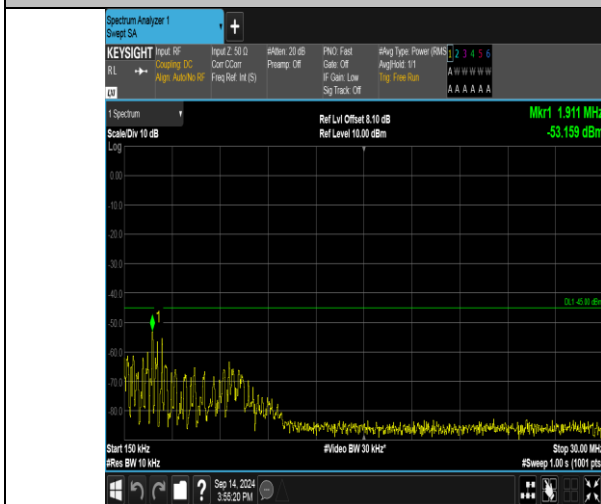
Band41_20MHz_16QAM_41140_1RB#99_0.15-30_0.15-30
