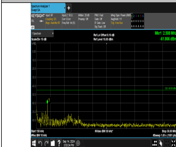
Band41_20MHz_16QAM_41140_1RB#0_0.15~30_0.15~30
