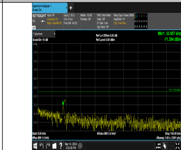
Band41_20MHz_16QAM_41140_1RB#0_0.009~0.15_0.009~0.15
