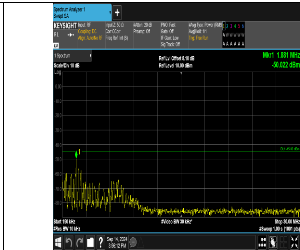
Band41_20MHz_QPSK_41140_100RB#0_0.15~30_0.15~30
