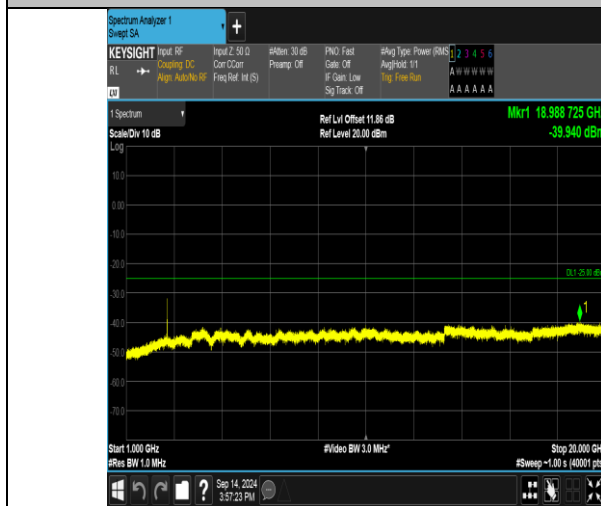
Band41_20MHz_16QAM_41140_100RB#0_1000~20000_1000~20000
