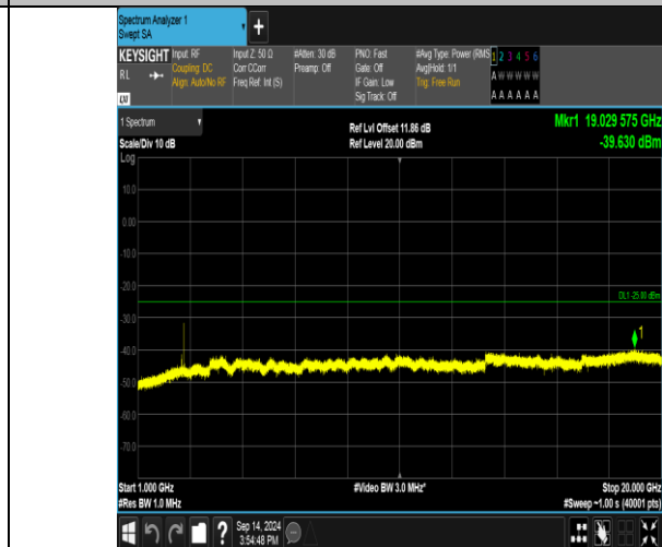
Band41_20MHz_QPSK_41140_1RB#99_1000-20000_1000-20000
