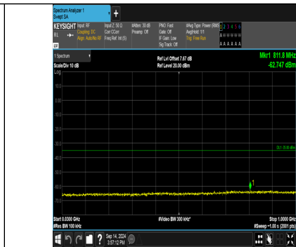
Band41_20MHz_16QAM_41140_100RB#0_30~1000_30~1000
