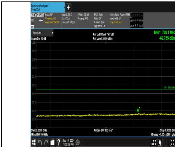
Band41_20MHz_QPSK_41140_1RB#0_30~1000_30~1000
