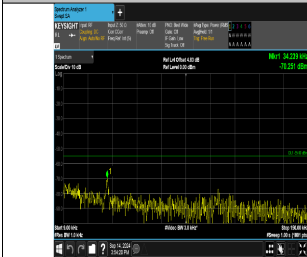
Band41_20MHz_QPSK_41140_1RB#99_0.009-0.15_0.009-0.15
