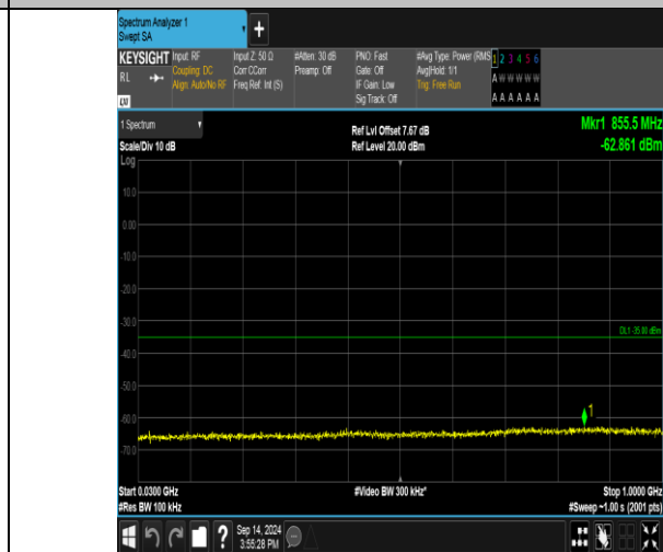
Band41_20MHz_16QAM_41140_1RB#99_30-1000_30-1000
