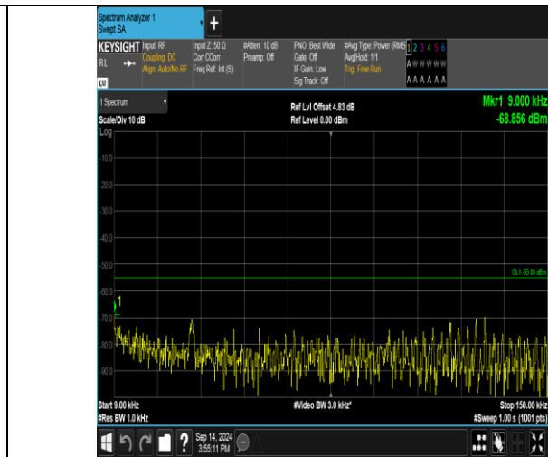
Band41_20MHz_16QAM_41140_1RB#99_0.009-0.15_0.009-0.15
