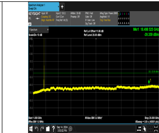
Band41_20MHz_QPSK_41140_1RB#0_1000~20000_1000~20000
