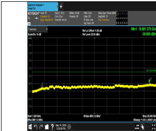
Band41_20MHz_16QAM_41140_1RB#0_1000-20000_1000-20000
