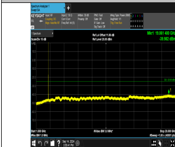
Band41_20MHz_16QAM_41140_1RB#99_1000-20000_1000-20000
