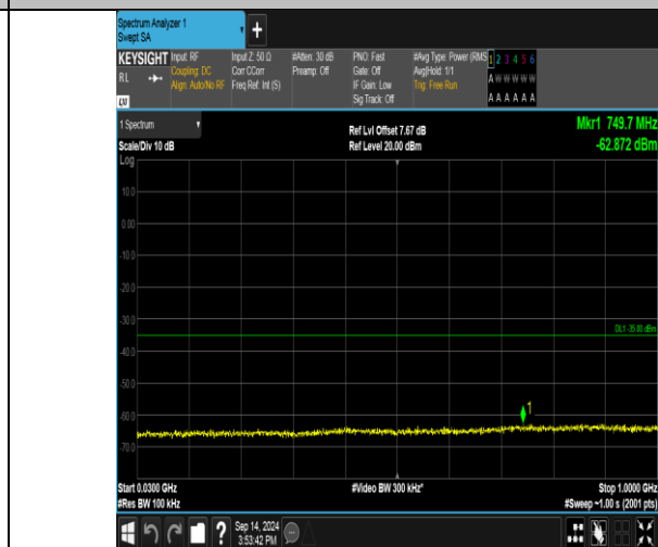
Band41_20MHz_16QAM_41140_1RB#0_30~1000_30~1000
