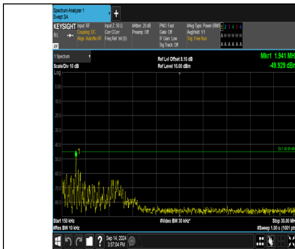
Band41_20MHz_16QAM_41140_100RB#0_0.15~30_0.15~30
