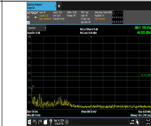
Band41_20MHz_QPSK_41140_1RB#99_0.15-30_0.15-30
