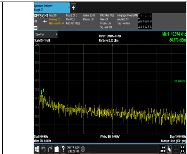
Band66_3MHz_16QAM_132322_15RB#0_0.009~0.15_0.009~0.15
