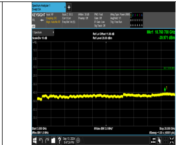
Band66_3MHz_16QAM_132322_1RB#14_3000~20000_3000~20000
