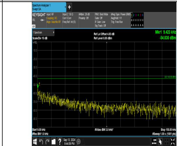
Band66_3MHz_16QAM_132322_1RB#0_0.009~0.15_0.009~0.15
