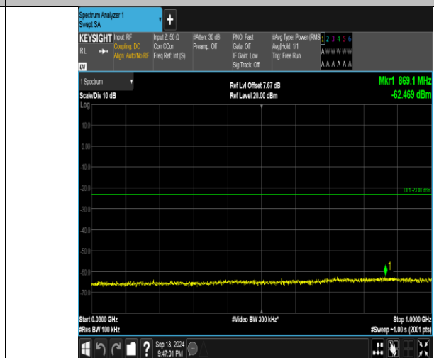
Band66_3MHz_16QAM_132322_1RB#14_30~1000_30~1000
