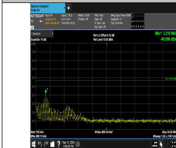
Band66_3MHz_16QAM_132322_1RB#14_0.15~30_0.15~30
