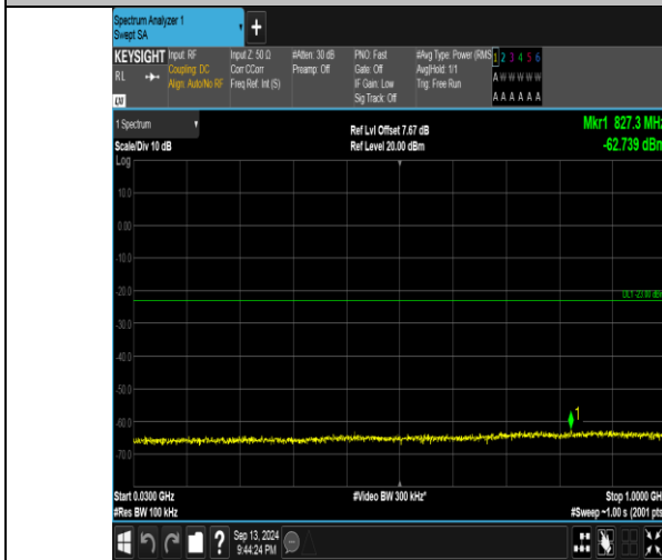
Band66_3MHz_QPSK_132322_1RB#0_30~1000_30~1000
