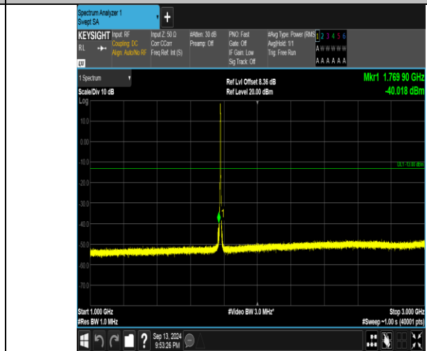
Band66_3MHz_QPSK_132657_15RB#0_1000~3000_1000~3000
