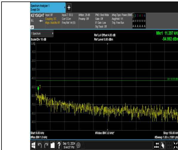
Band66_3MHz_QPSK_132322_1RB#0_0.009~0.15_0.009~0.15
