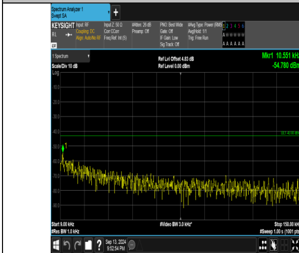
Band66_3MHz_QPSK_132657_15RB#0_0.009~0.15_0.009~0.15
