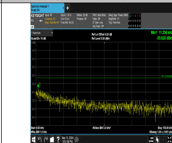
Band66_3MHz_16QAM_132657_1RB#14_0.009~0.15_0.009~0.15
