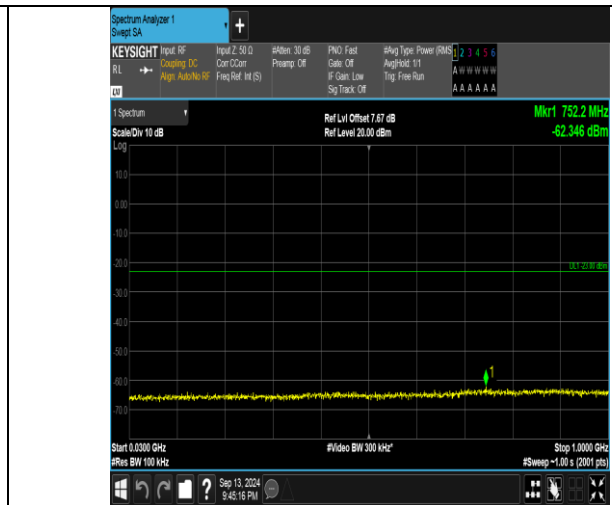
Band66_3MHz_16QAM_132322_1RB#0_30~1000_30~1000
