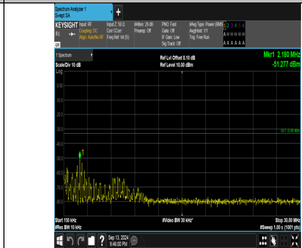
Band66_3MHz_QPSK_132322_1RB#14_0.15~30_0.15~30
