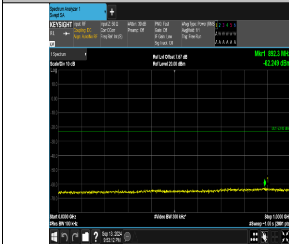
Band66_3MHz_QPSK_132657_15RB#0_30~1000_30~1000
