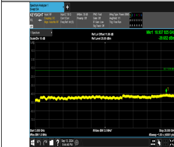
Band66_3MHz_QPSK_132322_1RB#0_3000~20000_3000~20000
