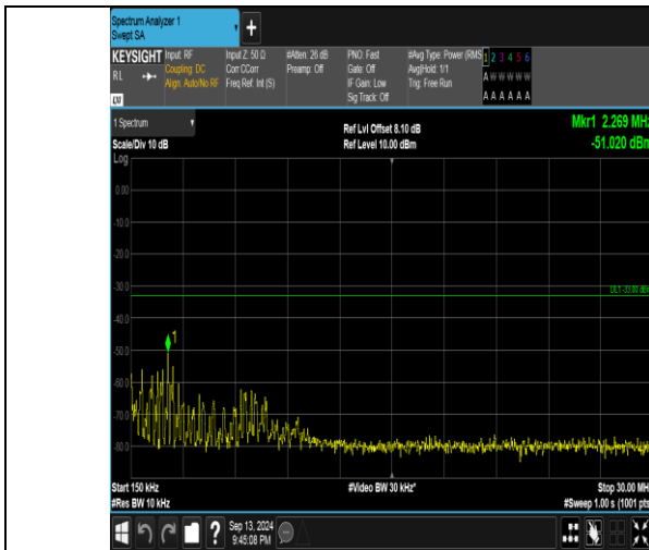
Band66_3MHz_16QAM_132322_1RB#0_0.15~30_0.15~30
