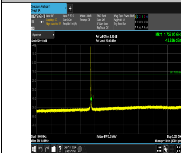
Band66_3MHz_16QAM_132322_15RB#0_1000~3000_1000~3000
