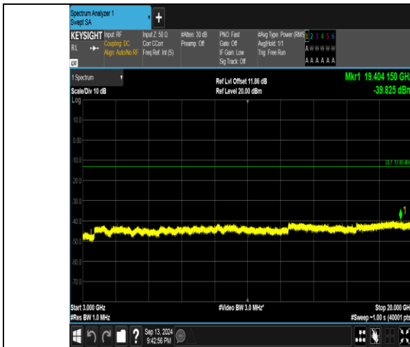
Band66_3MHz_QPSK_131987_15RB#0_3000~20000_3000~20000
