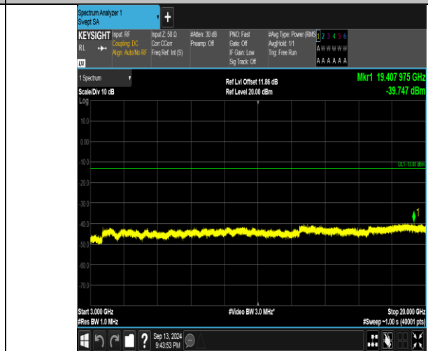
Band66_3MHz_16QAM_131987_15RB#0_3000~20000_3000~20000
