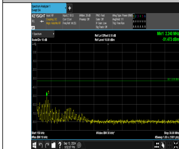
Band66_3MHz_16QAM_132657_1RB#14_0.15~30_0.15~30
