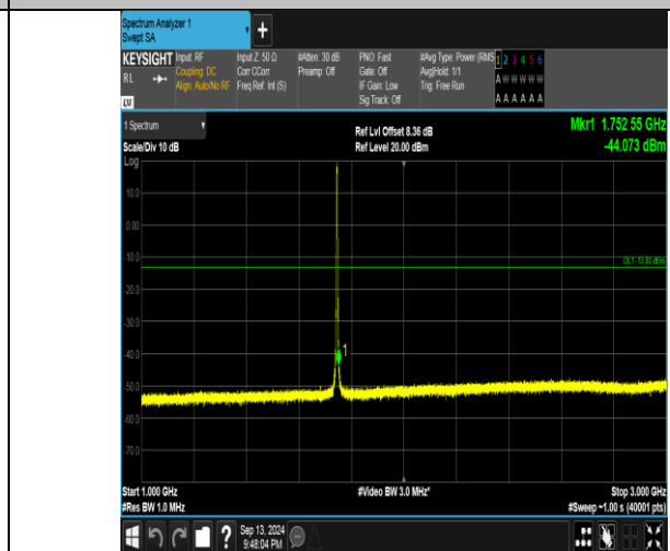
Band66_3MHz_QPSK_132322_15RB#0_1000~3000_1000~3000
