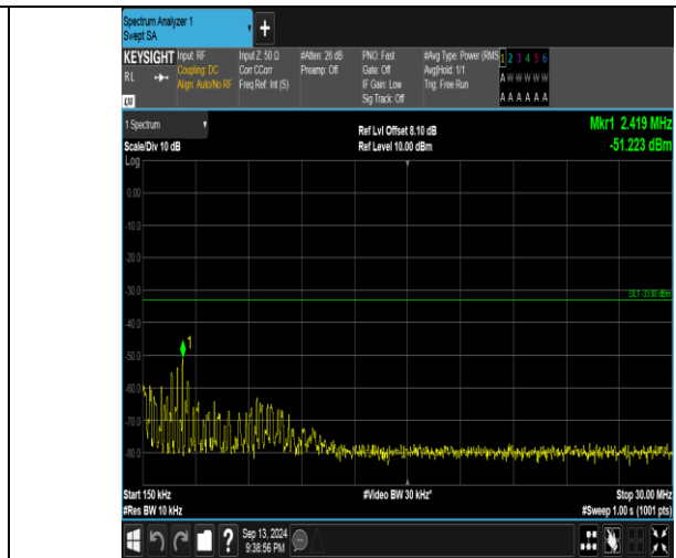
Band66_3MHz_QPSK_131987_1RB#0_0.15~30_0.15~30
