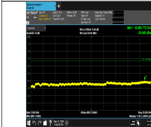
Band66_3MHz_QPSK_132322_1RB#14_3000~20000_3000~20000
