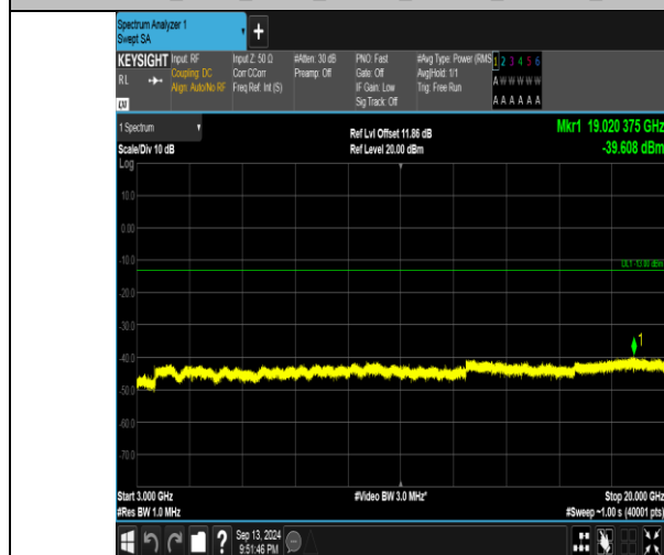
Band66_3MHz_QPSK_132657_1RB#14_3000~20000_3000~20000
