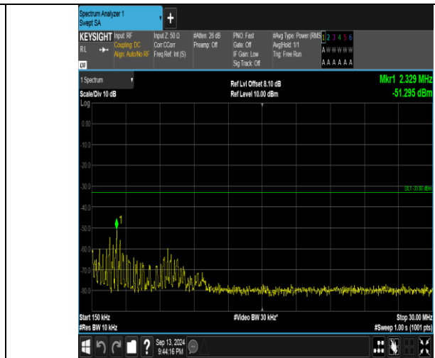
Band66_3MHz_QPSK_132322_1RB#0_0.15~30_0.15~30
