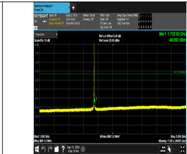
Band66_3MHz_QPSK_132322_1RB#14_1000~3000_1000~3000
