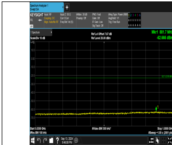
Band66_3MHz_QPSK_132322_1RB#14_30~1000_30~1000
