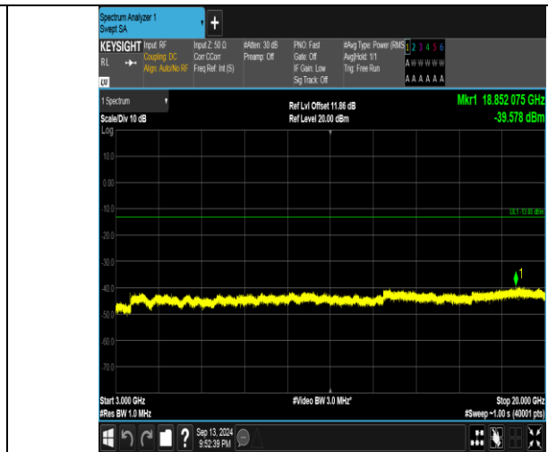
Band66_3MHz_16QAM_132657_1RB#14_3000~20000_3000~20000
