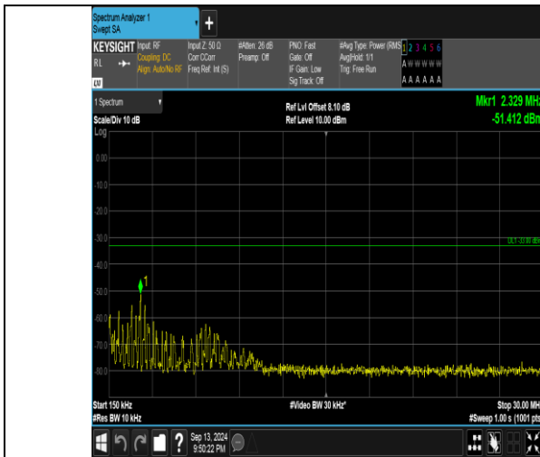
Band66_3MHz_16QAM_132657_1RB#0_0.15~30_0.15~30
