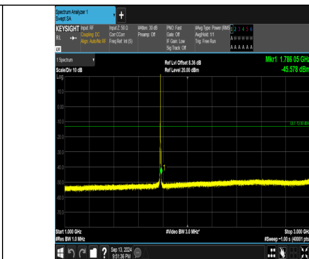
Band66_3MHz_QPSK_132657_1RB#14_1000~3000_1000~3000
