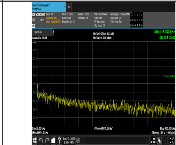
Band66_3MHz_16QAM_132322_1RB#14_0.009~0.15_0.009~0.15
