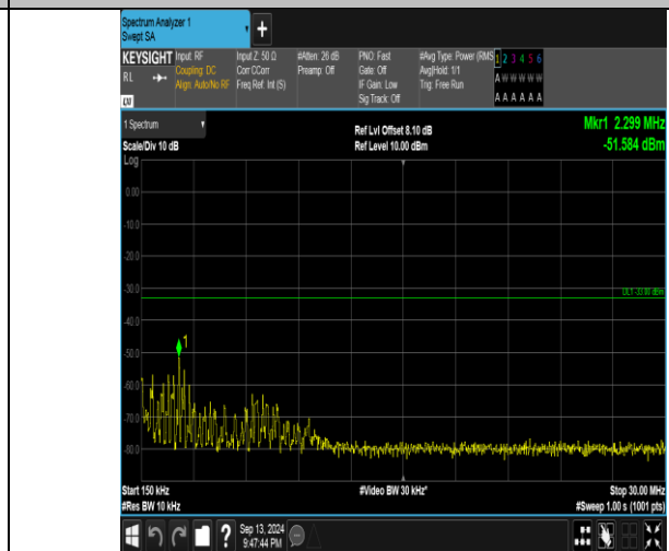
Band66_3MHz_QPSK_132322_15RB#0_0.15~30_0.15~30
