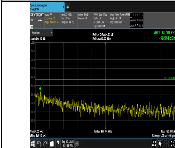
Band66_3MHz_QPSK_132657_1RB#14_0.009~0.15_0.009~0.15
