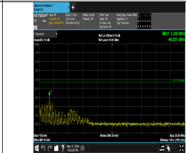
Band66_3MHz_QPSK_131987_15RB#0_0.15~30_0.15~30
