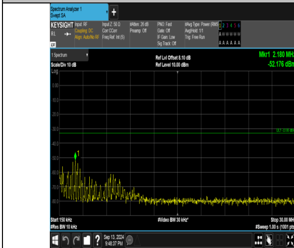
Band66_3MHz_16QAM_132322_15RB#0_0.15~30_0.15~30
