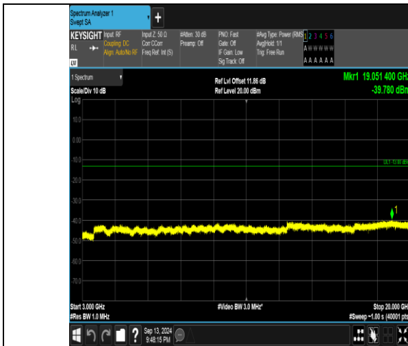
Band66_3MHz_QPSK_132322_15RB#0_3000~20000_3000~20000
