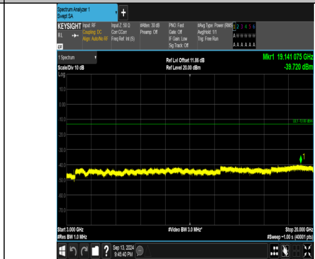
Band66_3MHz_16QAM_132322_1RB#0_3000~20000_3000~20000
