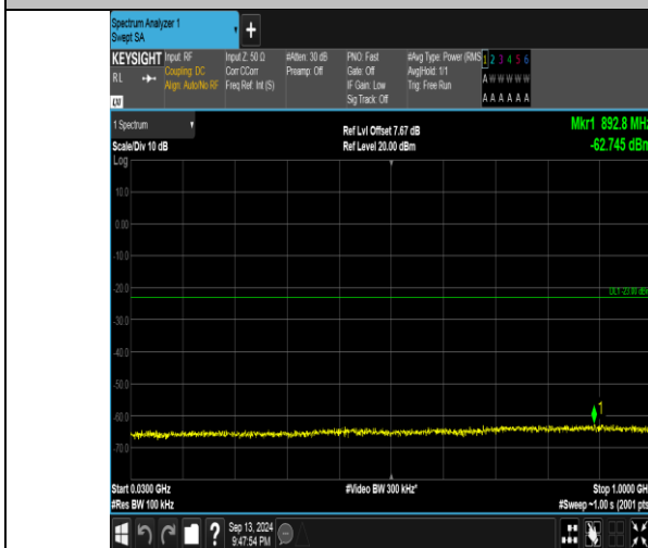
Band66_3MHz_QPSK_132322_15RB#0_30~1000_30~1000
