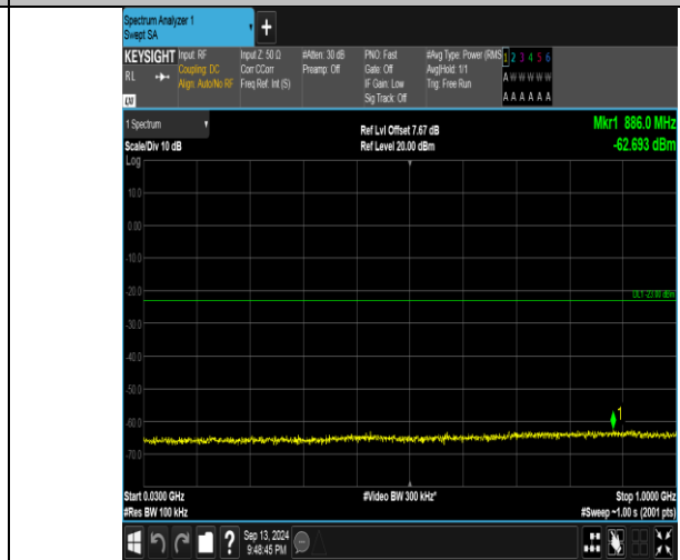
Band66_3MHz_16QAM_132322_15RB#0_30~1000_30~1000
