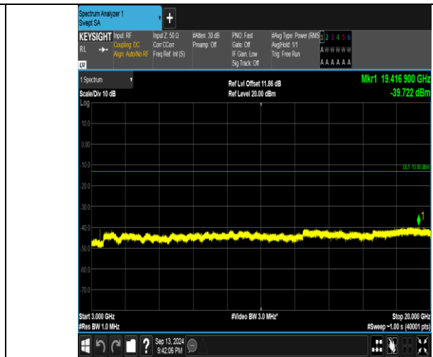
Band66_3MHz_16QAM_131987_1RB#14_3000~20000_3000~20000
