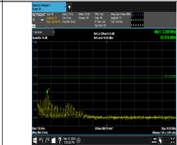
Band66_3MHz_QPSK_132657_15RB#0_0.15~30_0.15~30
