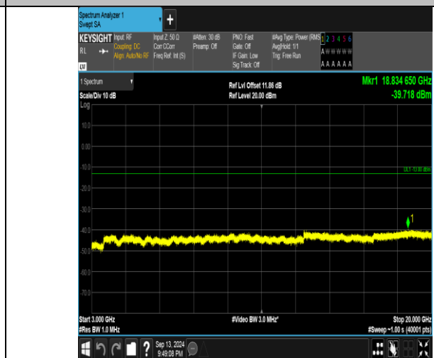
Band66_3MHz_16QAM_132322_15RB#0_3000~20000_3000~20000
