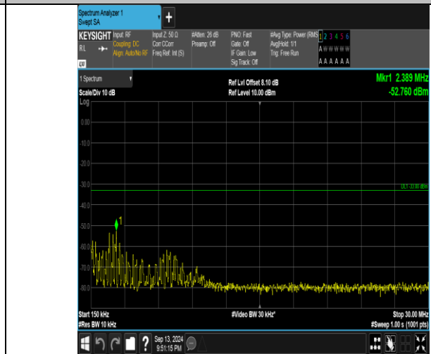
Band66_3MHz_QPSK_132657_1RB#14_0.15~30_0.15~30
