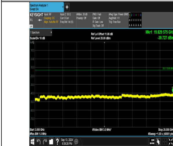
Band66_3MHz_QPSK_131987_1RB#0_3000~20000_3000~20000
