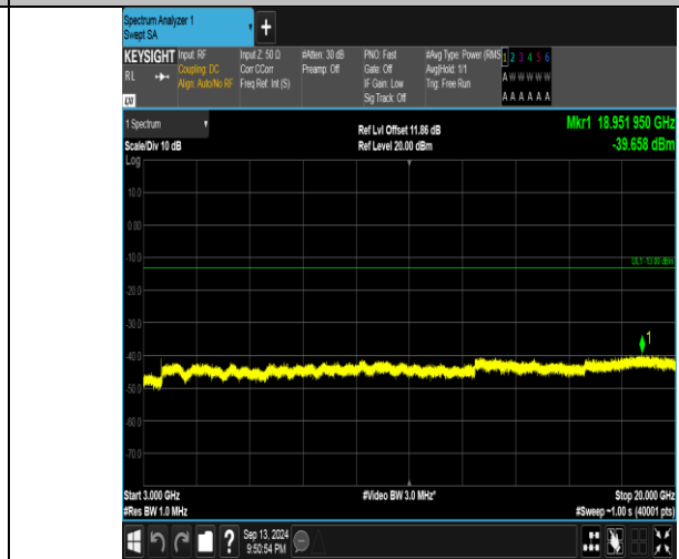
Band66_3MHz_16QAM_132657_1RB#0_3000~20000_3000~20000
