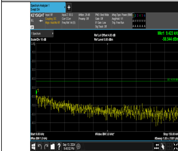
Band66_3MHz_QPSK_132322_1RB#14_0.009~0.15_0.009~0.15
