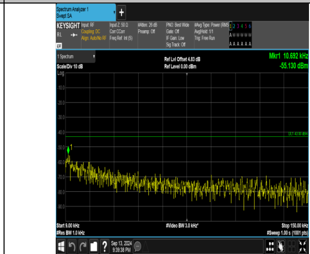
Band66_3MHz_16QAM_131987_1RB#0_0.009~0.15_0.009~0.15
