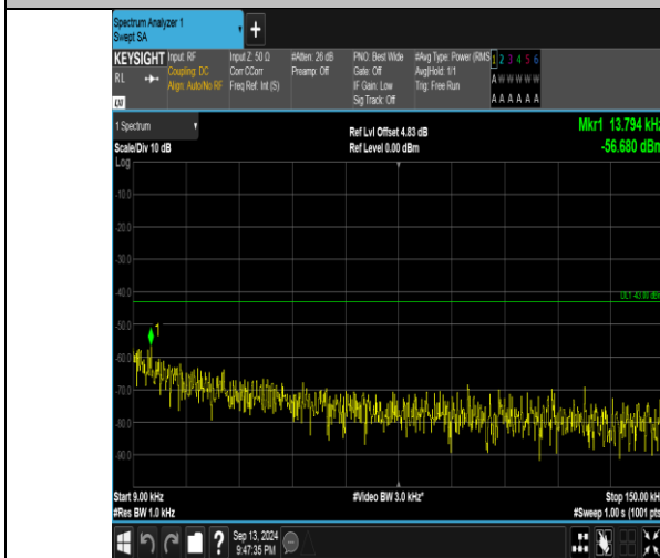
Band66_3MHz_QPSK_132322_15RB#0_0.009~0.15_0.009~0.15
