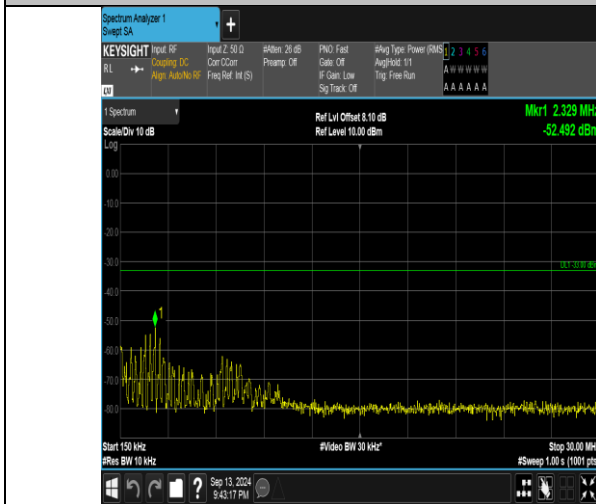
Band66_3MHz_16QAM_131987_15RB#0_0.15~30_0.15~30
