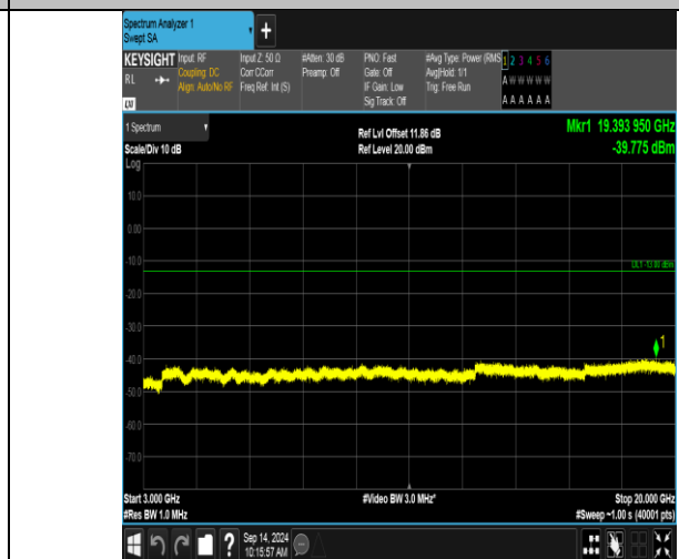
Band66_20MHz_16QAM_132572_100RB#0_3000~20000_3000~20000
