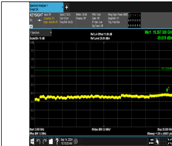
Band66_20MHz_QPSK_132572_100RB#0_3000~20000_3000~20000
