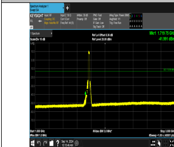
Band66_20MHz_16QAM_132572_100RB#0_1000~3000_1000~3000
