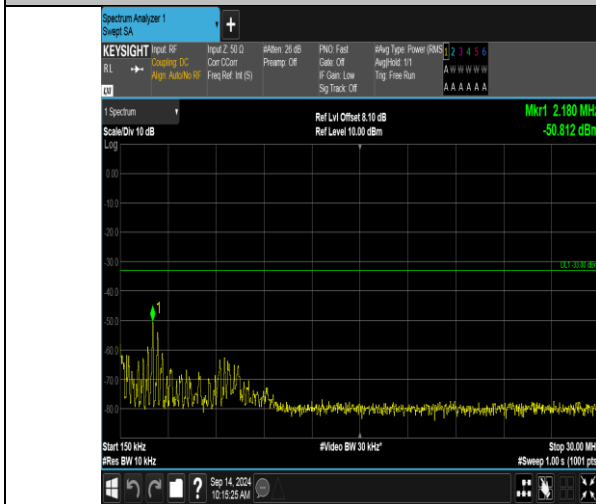
Band66_20MHz_16QAM_132572_100RB#0_0.15~30_0.15~30
