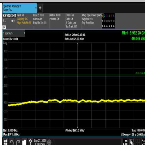
Band5-4233-5-1000~10000MHz-PASS
