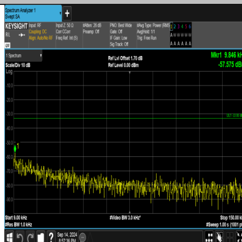
Band5-4233-2-0.009~0.15MHz-PASS
