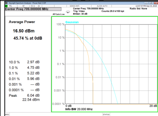
Band17_1_QPSK_Middle
