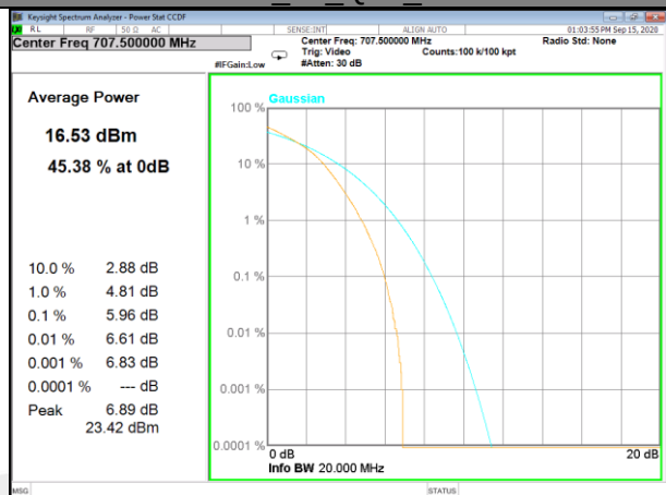
Band12_50_QPSK_High
