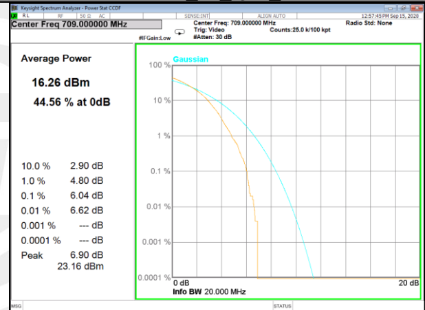
Band17_50_QPSK_Middle
