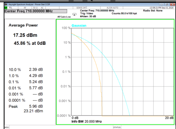
Band17_50_QPSK_Middle
