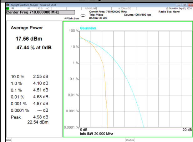
Band17_1_QPSK_Middle
