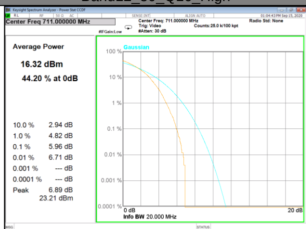
Band12_50_Q16_High
