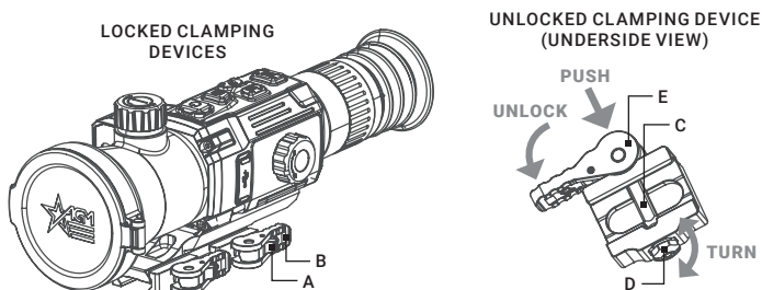
FIGURE 2-5. MOUNT
