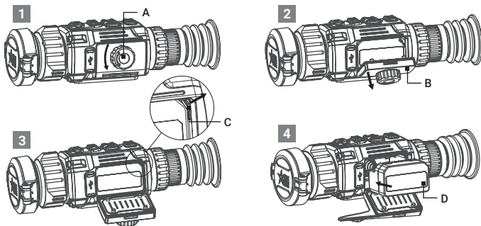
FIGURE 2-1. BATTERY INSTALLATION
