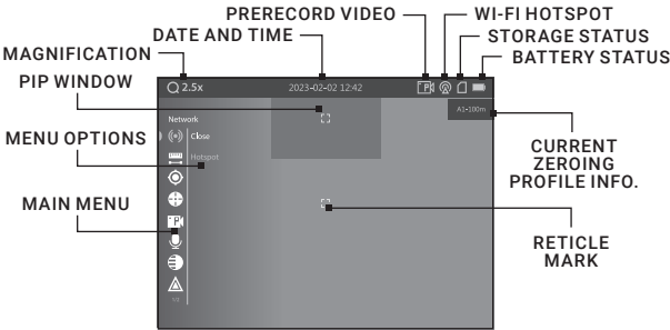
FIGURE 2-3. ON-SCREEN DISPLAY
