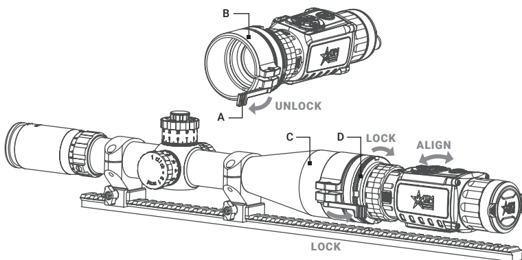
FIGURE 2-7. CLIP-ON INSTALLATION
