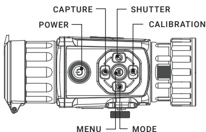
FIGURE 2-3. CONTROL BUTTONS
