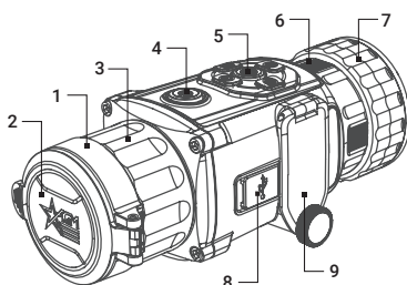
FIGURE 1-1. MAIN PARTS
