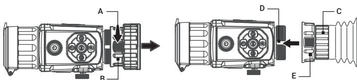
FIGURE 2-10. EYEPiece REPLACEMENT
