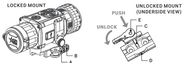
FIGURE 2-9. OPERATION OF THE QR MOUNT
