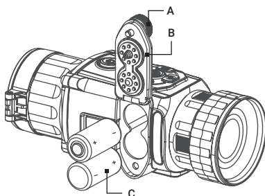
FIGURE 2-1. BATTERY INSTALLATION
