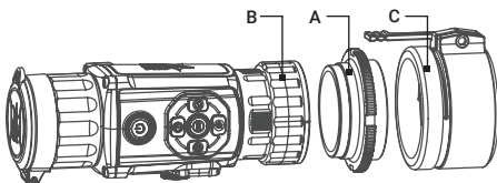
FIGURE 2-6. FRONT Q-R ADAPTER INSTALLATION
