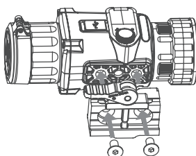
FIGURE 2-8. QUICK RELEASE MOUNT INSTALLATION
