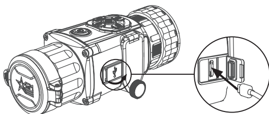
FIGURE 2-2. CABLE INTERFACE
