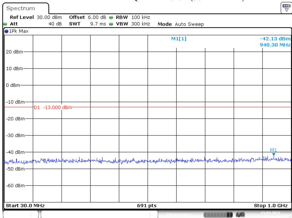
Band 2 1.4 MHz Low QPSK RB6#0 1(30MHz-1GHz)
