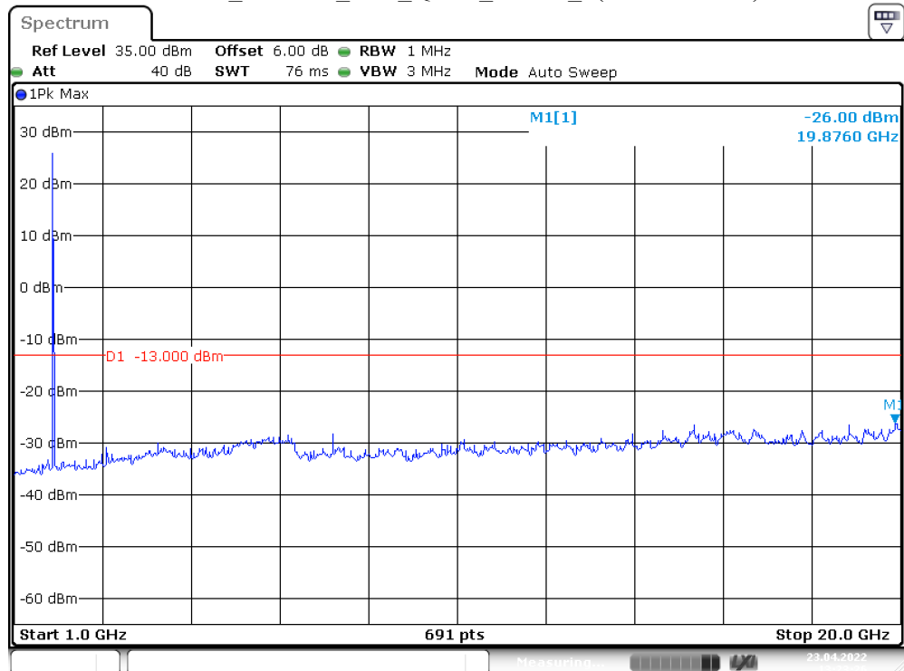
Band 2_1.4 MHz_Low_QPSK_RB6#0_2(1GHz-20GHz)
