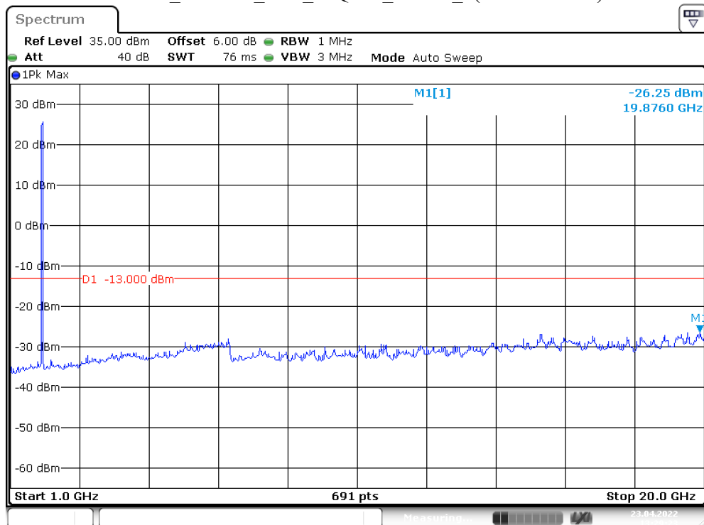
Band 2_1.4 MHz_Low_16QAM_RB6#0_2(1GHz-20GHz)
