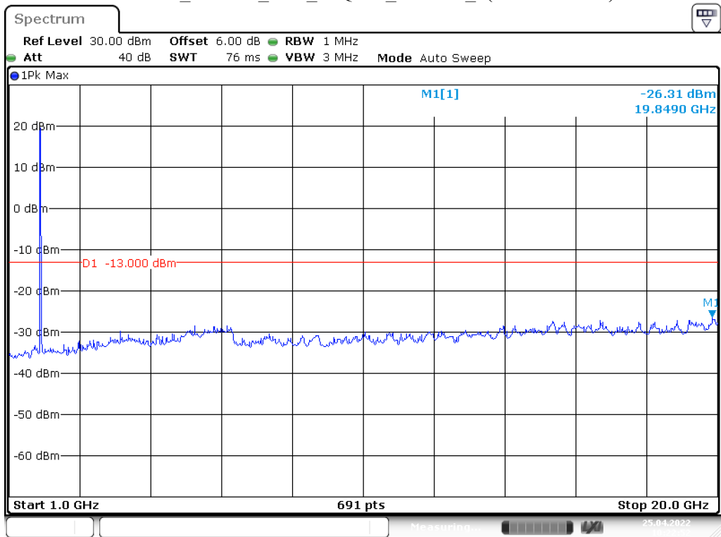
Band 25_15 MHz_Low_16QAM_RB75#0_2(1GHz-20GHz)
