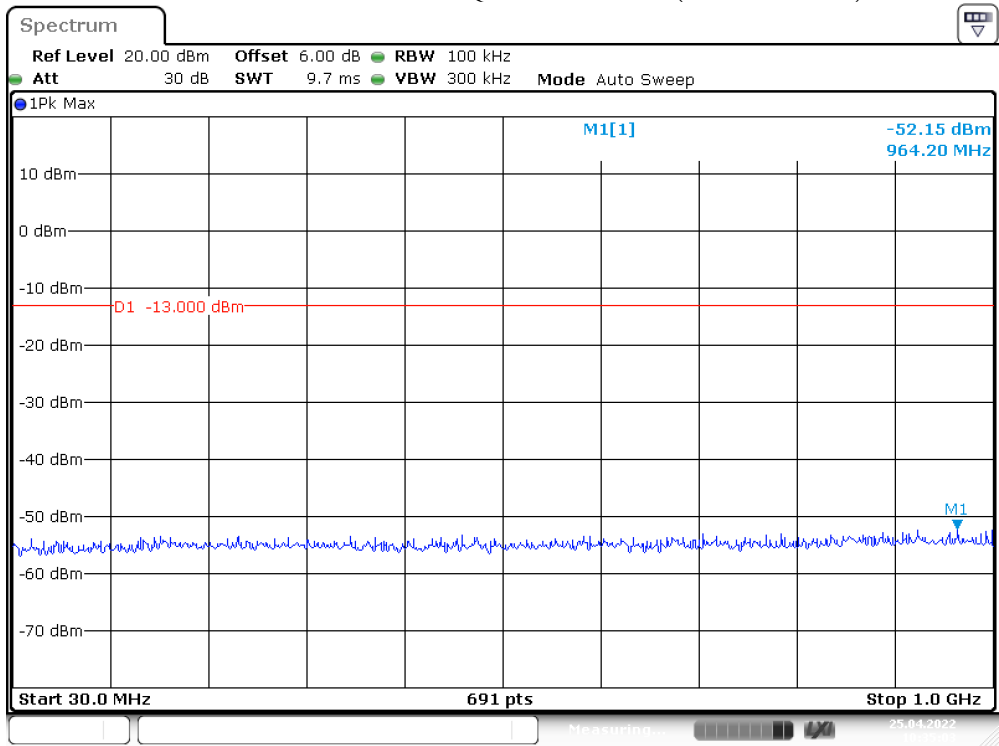
Band 25 15 MHz Low 16QAM RB75#0 1(30MHz-1GHz)
