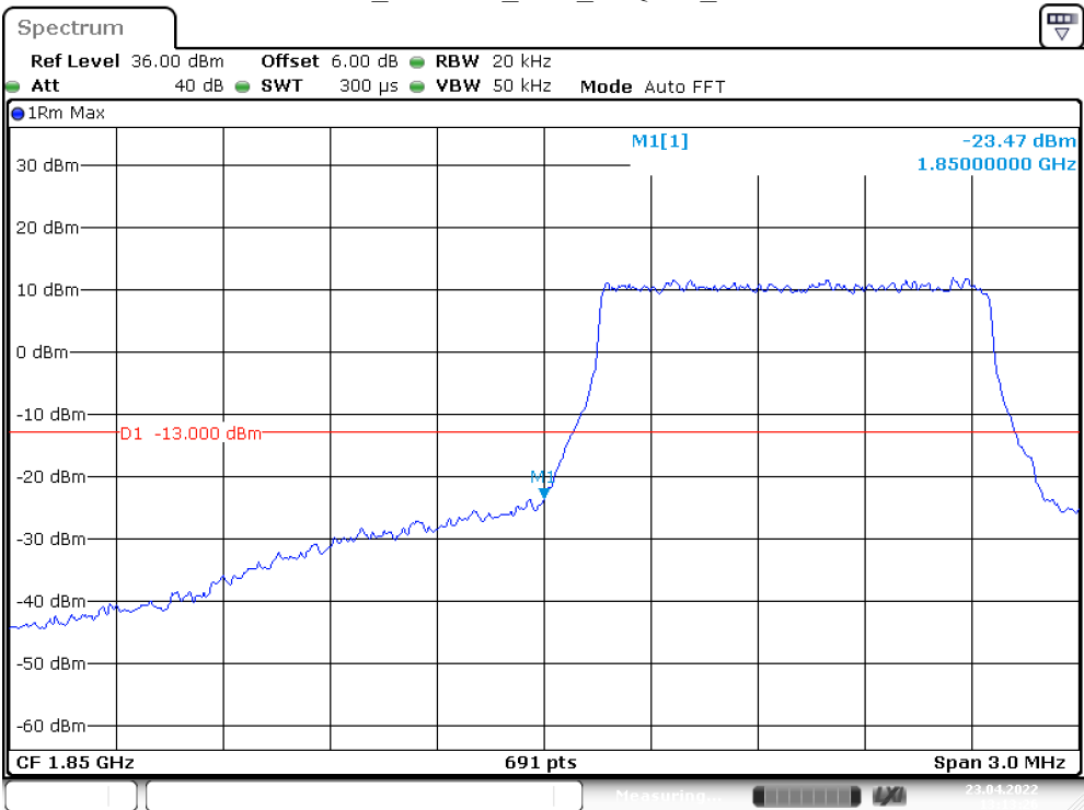
Band 2_1.4 MHz_Low_16QAM_RB6#0
