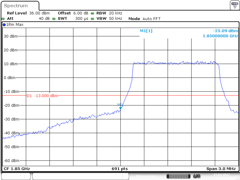
Band 2 1.4 MHz Low QPSK RB6#0
