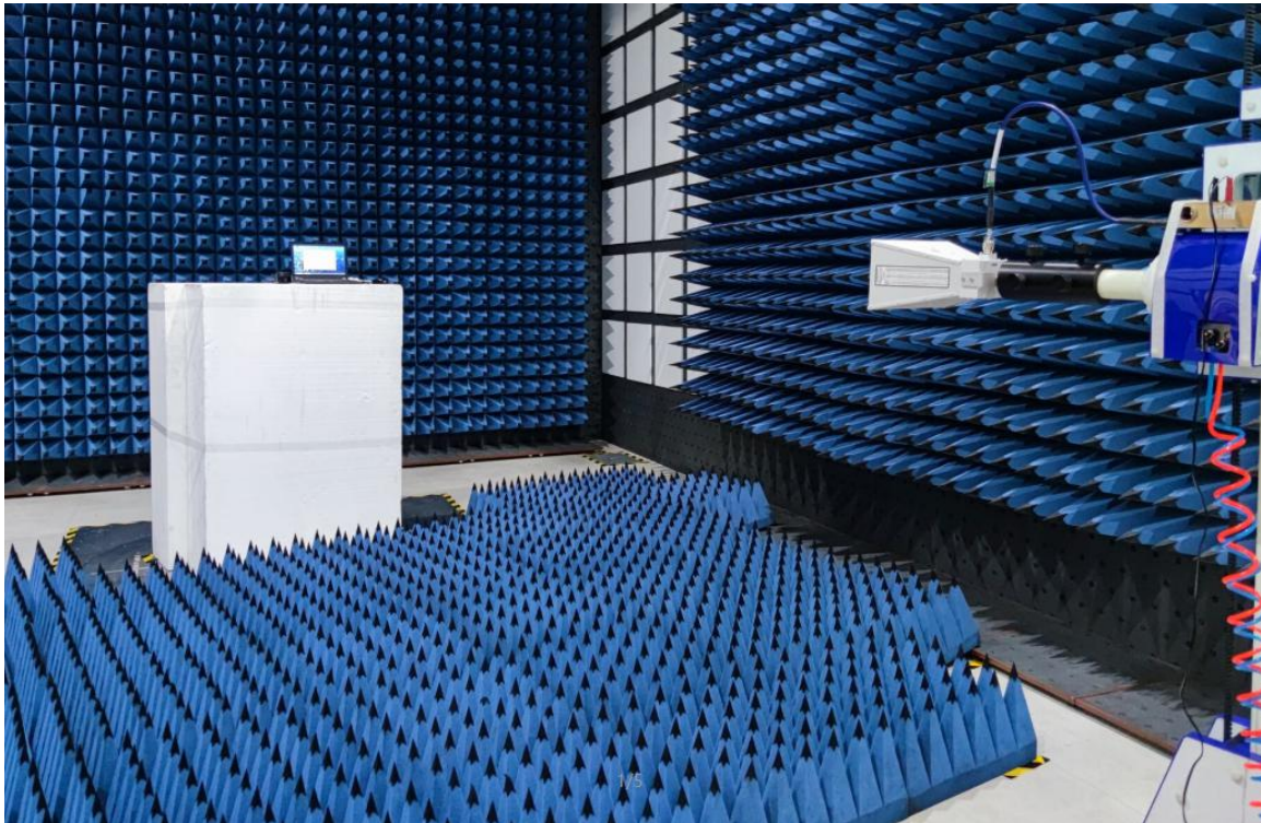
Above 1GHz
