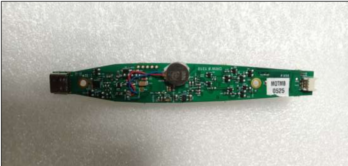
Photo: PCB Back View
