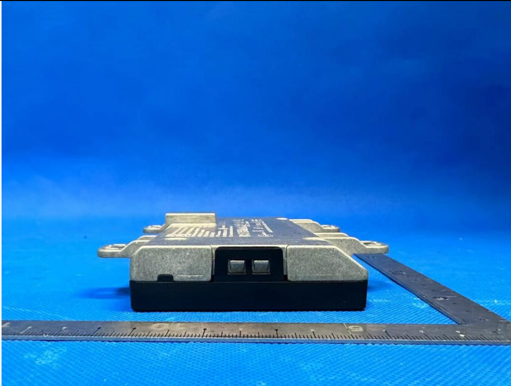
(10) EUT Photo(WPC014&WPC014-1)
