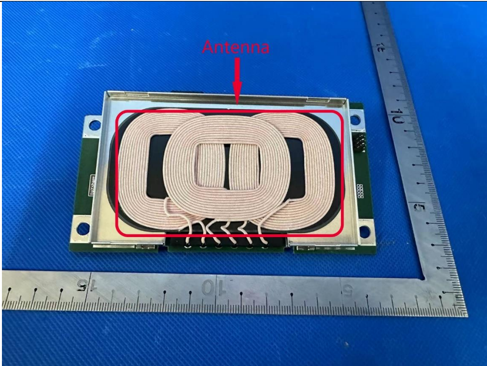
(4) EUT Photo(WPC013)
