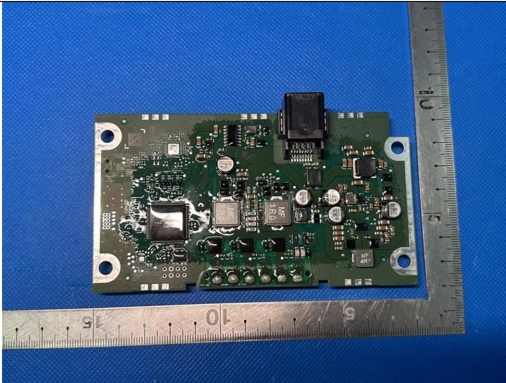
(10) EUT Photo(WPC014)
