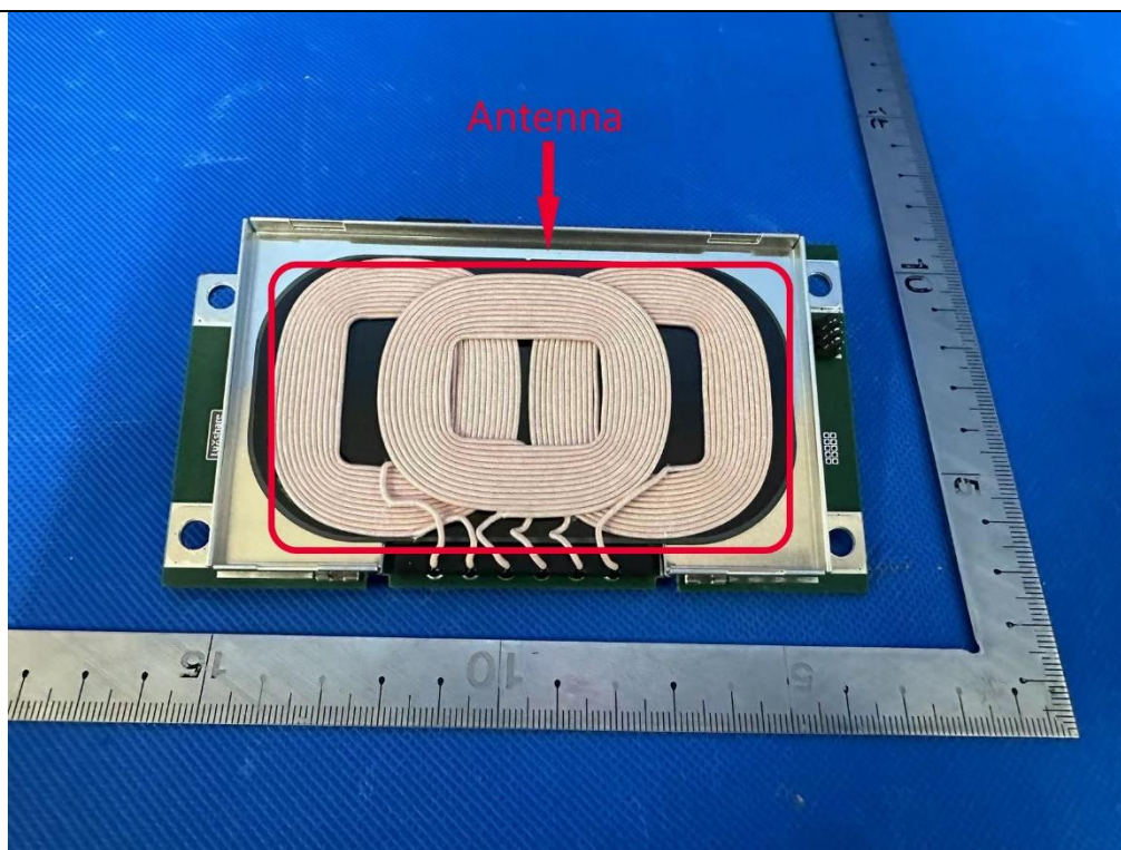
(11) EUT Photo(WPC014)
