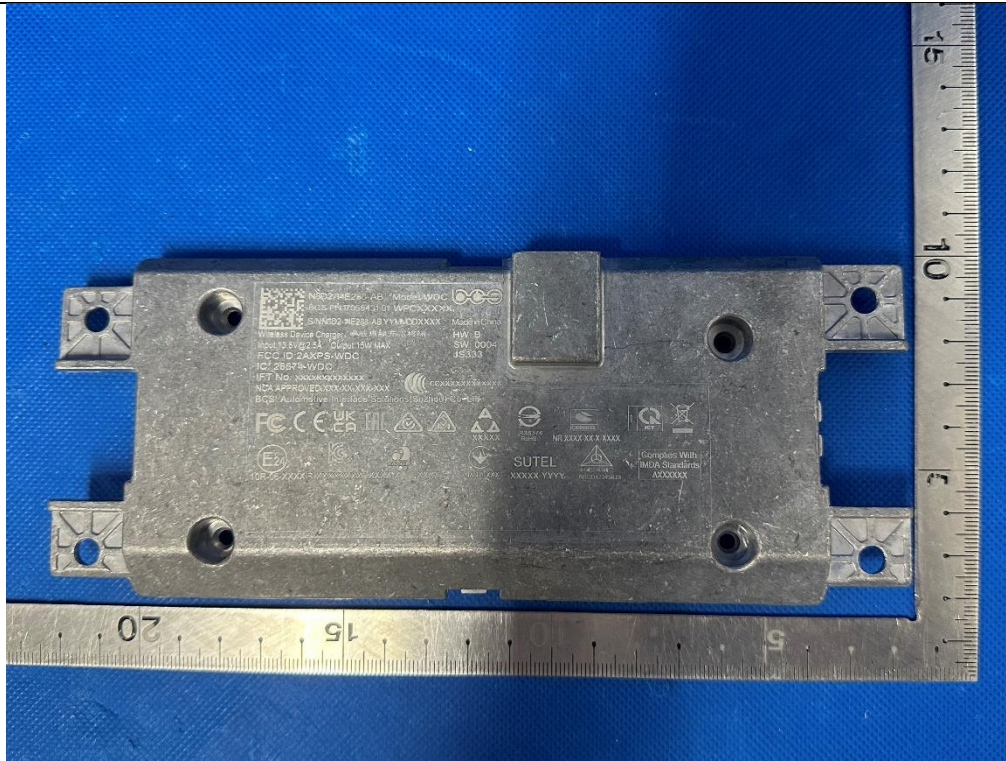
(2) EUT Photo(WPC013)
