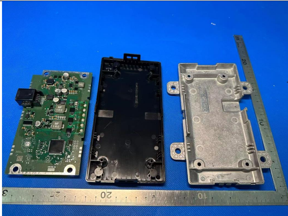
(8) EUT Photo(WPC014)
