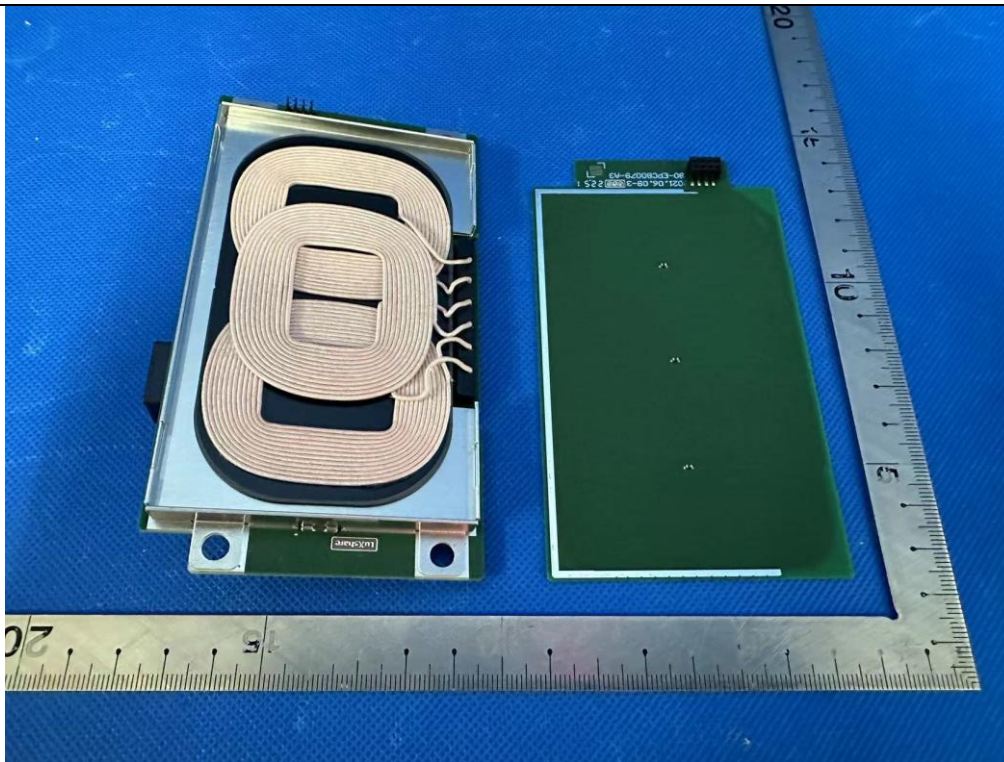
(4) EUT Photo(WPC013)
