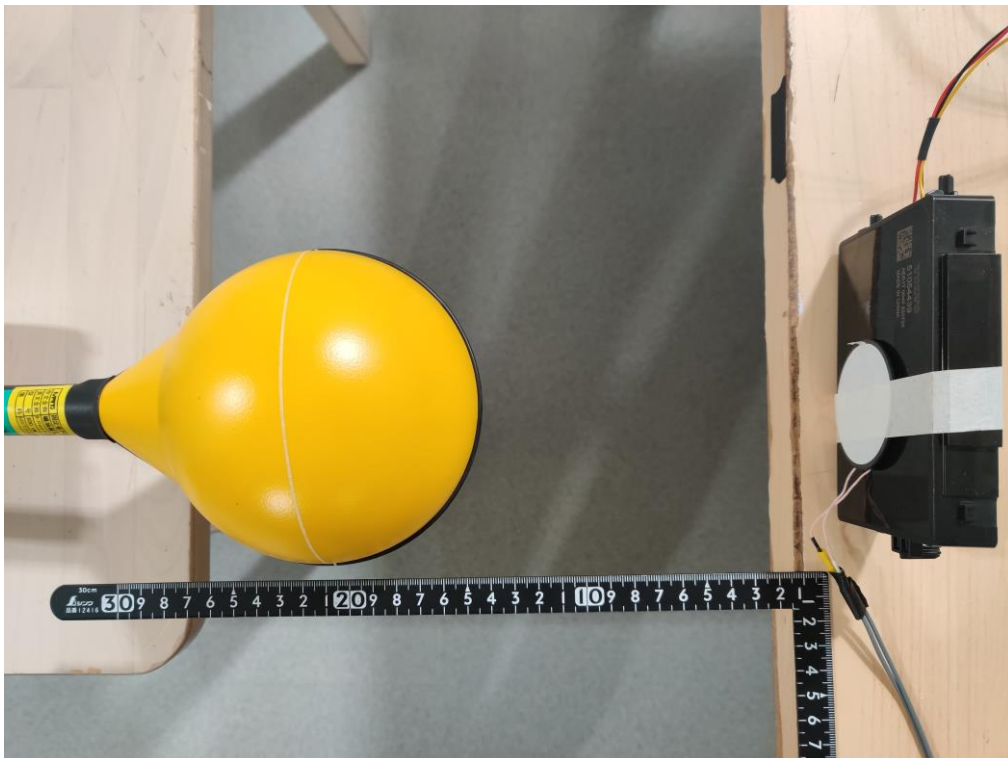
Description: RF Exposure Test Setup for Magnetic Field Emissions Test Mode 2
